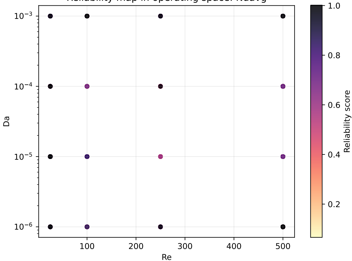
Reliability map in operating space: Nuavg
