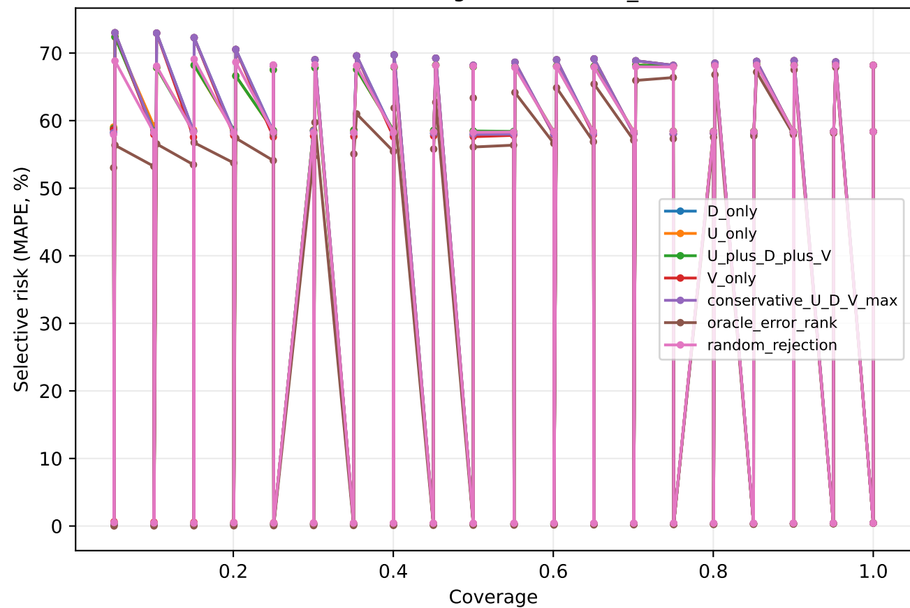
Risk-coverage curves: DelP_Pa
