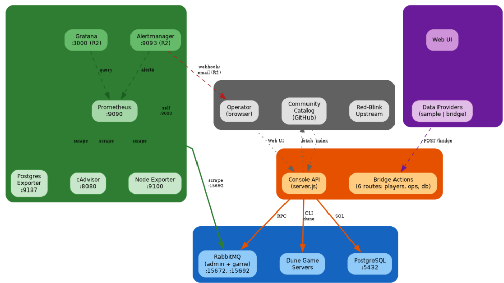
System architecture: Game Stack, Metrics Stack, Console API, Addon
