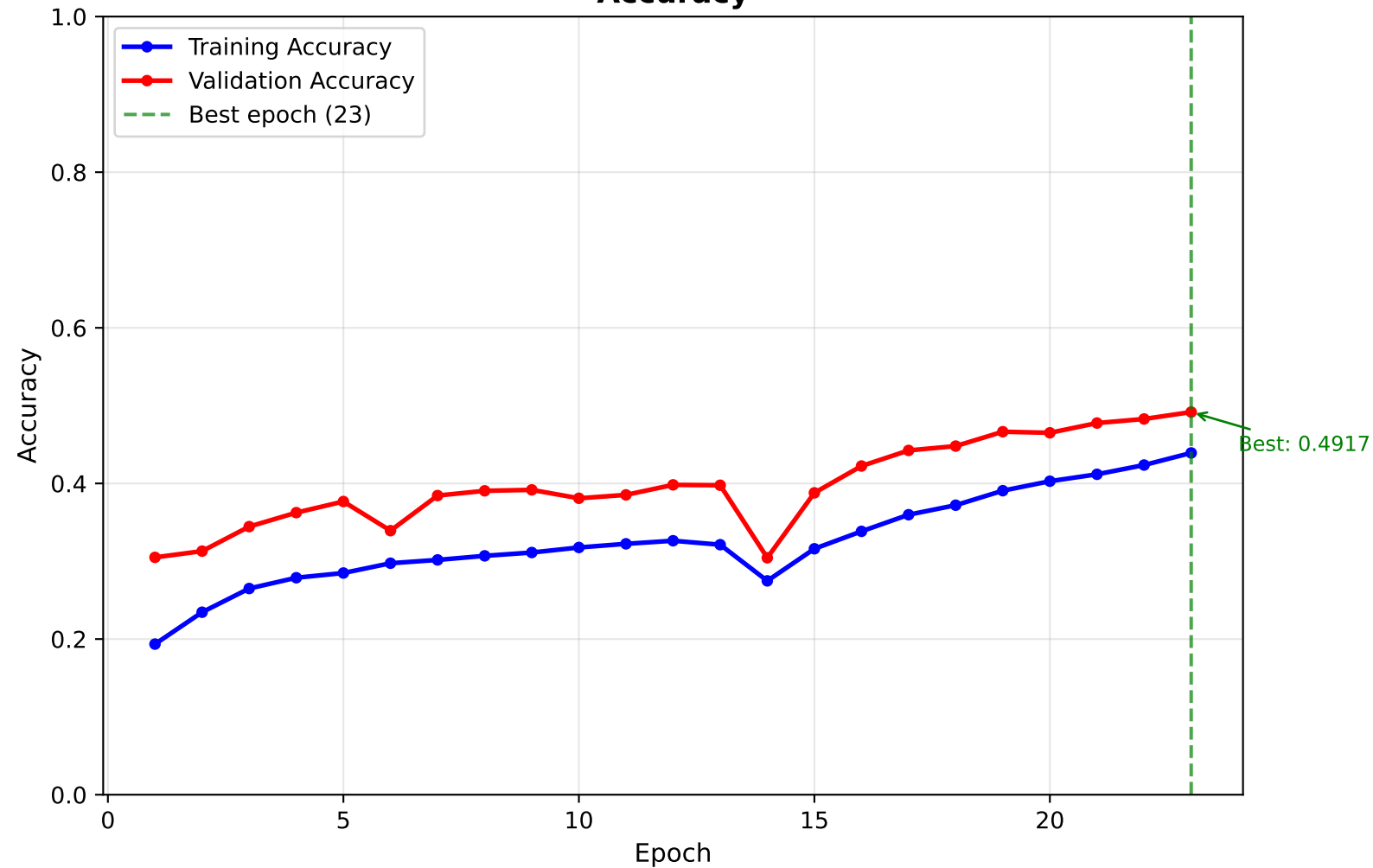
Accuracy
