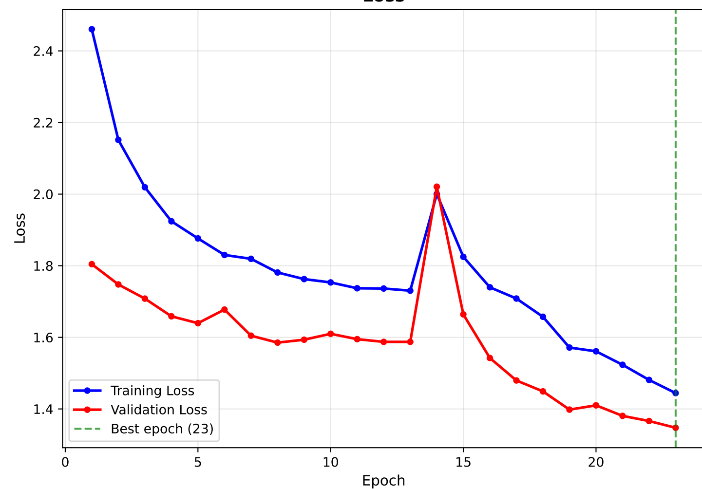
Loss
