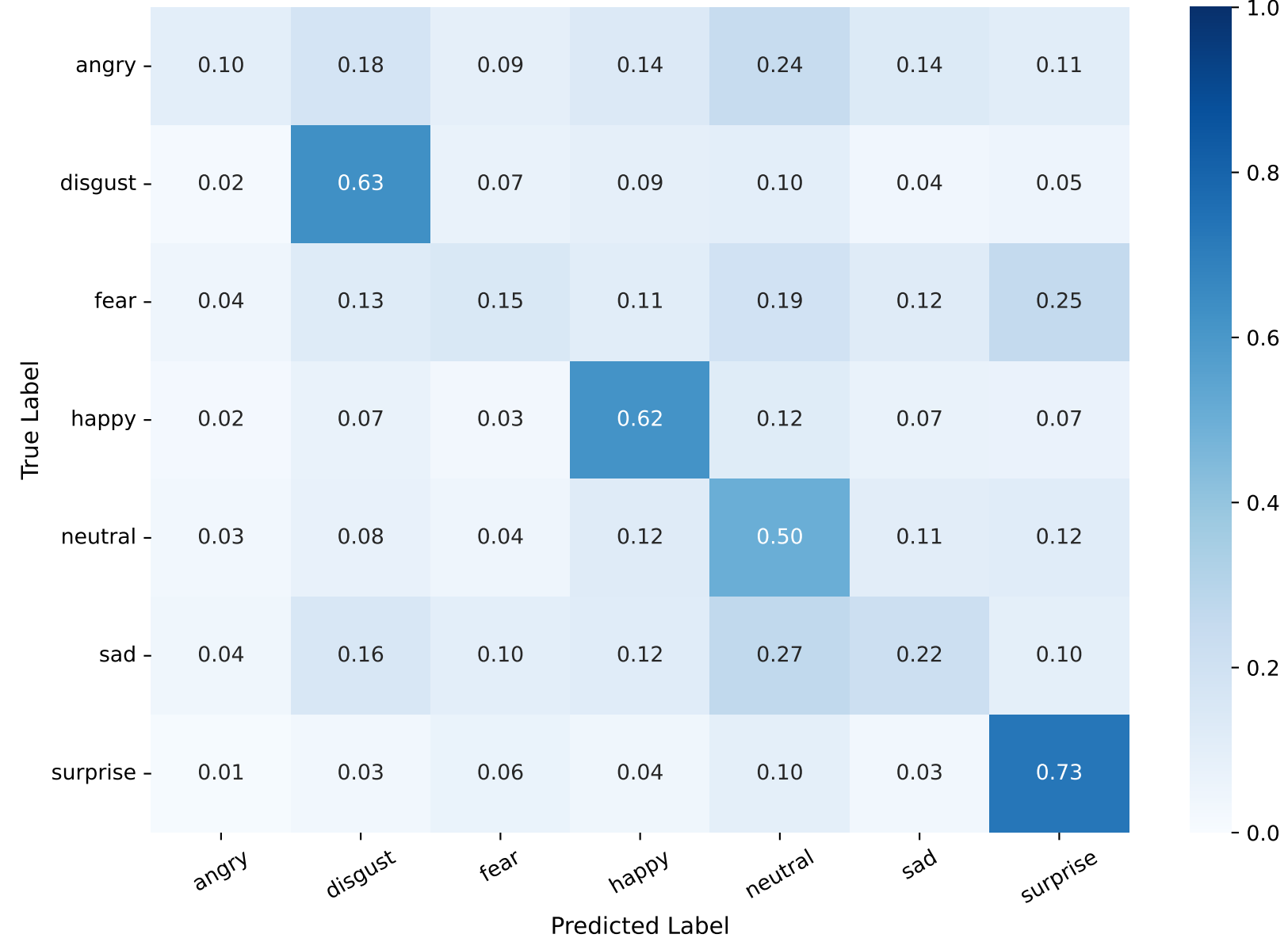
Normalized (Row %)
