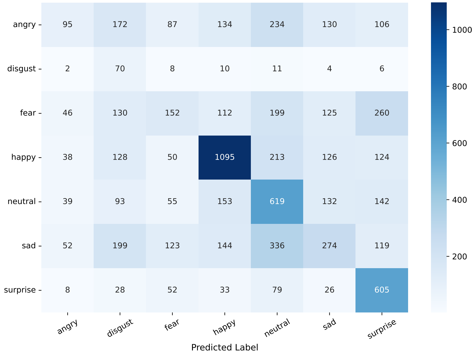
Raw Counts
