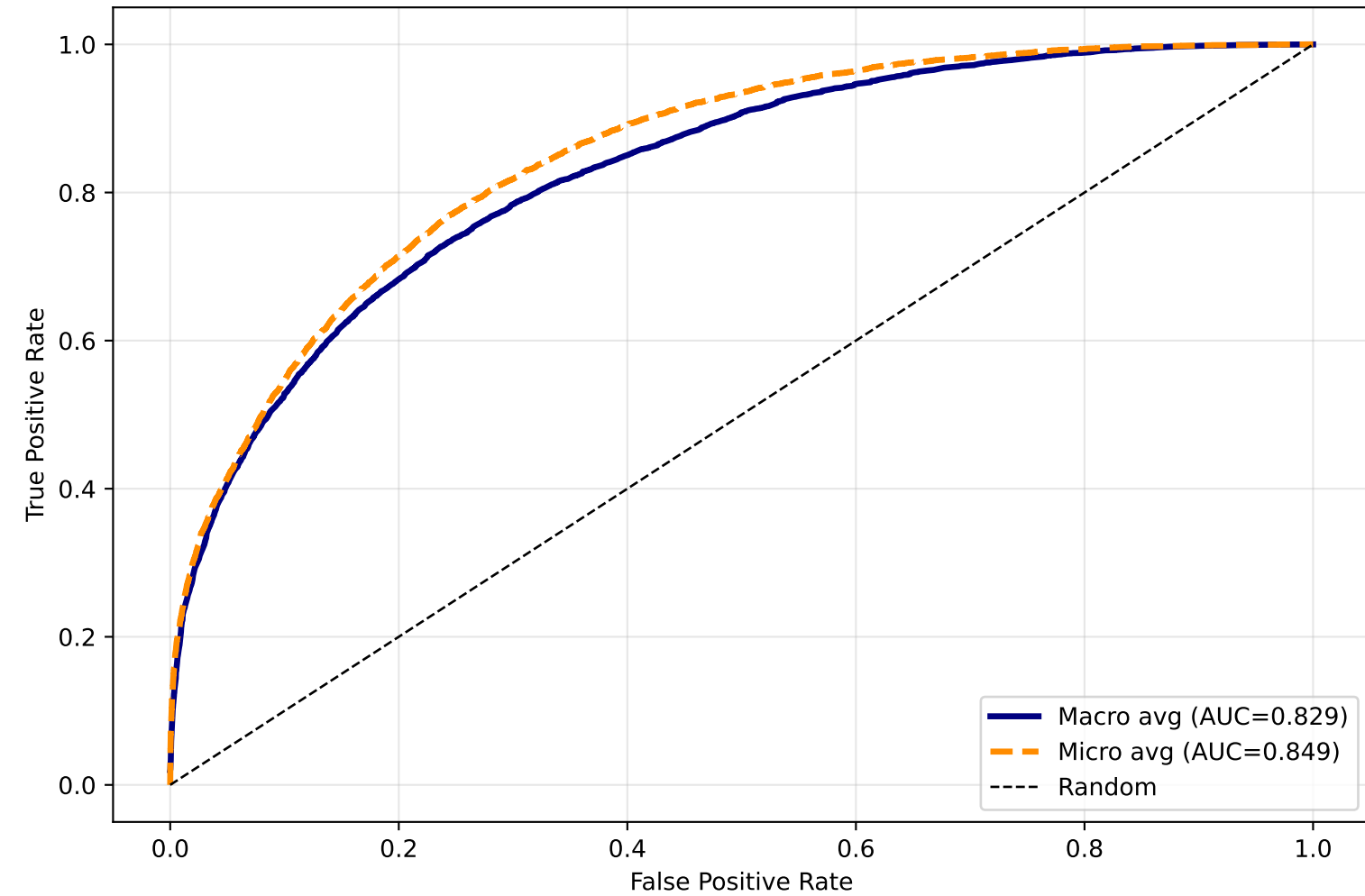
Macro & Micro Average ROC
