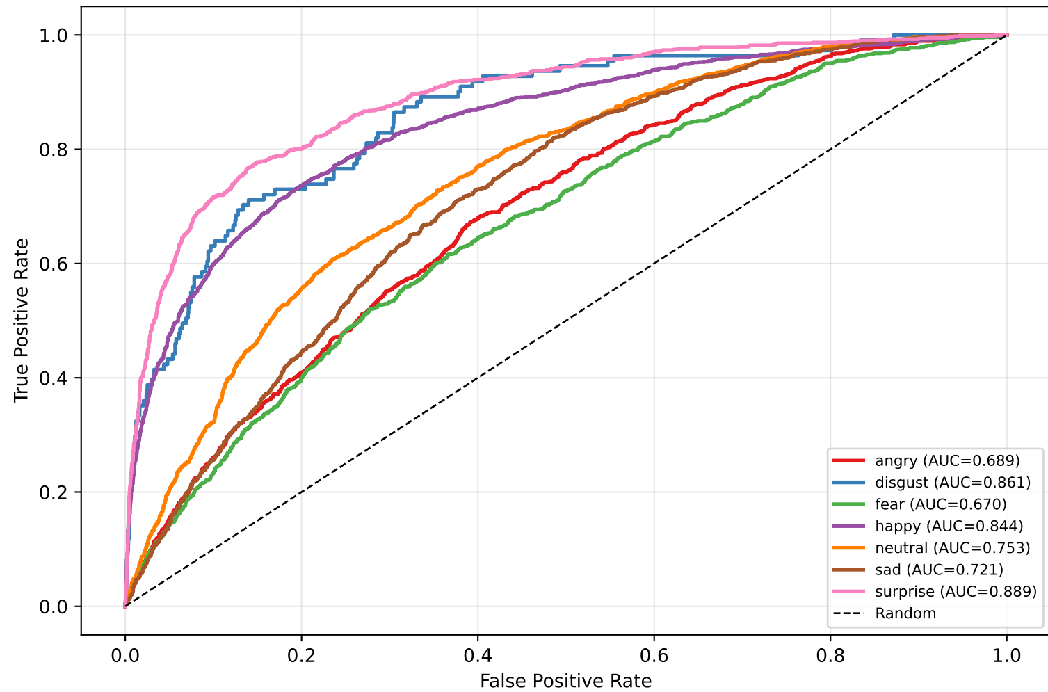
Per-Class ROC Curves
