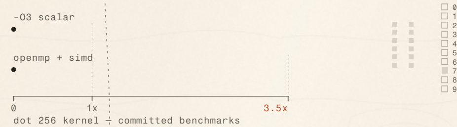
fig. 5.1 – the race – equal time, measured distance · and the forward pass, drawn. 3.5x – openmp+simd dot kernel vs -03 baseline (dot 256), committed benchmarks · avx-512 · avx2 · neon · wasm-simd128
