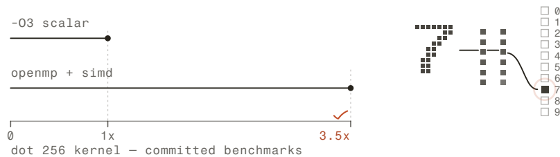
fig. 5.1 – the race – equal time, measured distance · and the forward pass, drawn. 3.5x – openmp+simd dot kernel vs -O3 baseline (dot 256), committed benchmarks · avx-512 · avx2 · neon · wasm-simd128
