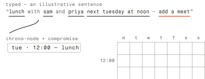
fig. 5.3 – the parse – a plain-english sentence resolves into chips on the week grid + a google meet link. chrono-node + compromise · google meet – multi-attendee invites · 1,145 tests passing – taskflow-calendar @ 69a59e7
