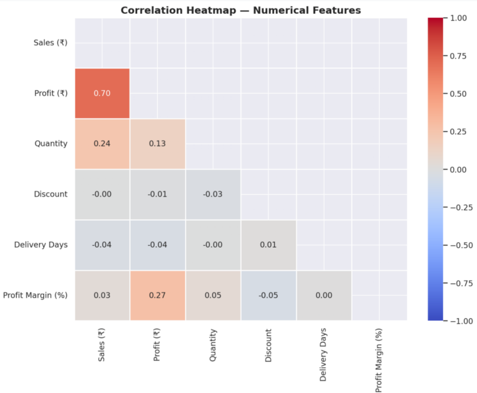
Fig 10: Correlation Heatmap
