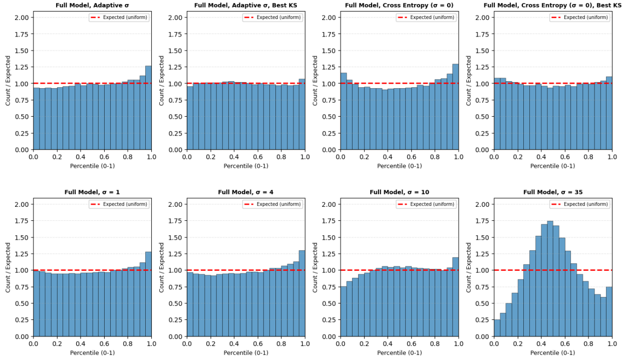
Figure 3: Quantile calibration emphasizing where predicted densities concentrate. Note that small \sigma values concentrate predictions at the extremes suggesting model overconfidence whereas large \sigma values appear underconfident with larger probability mass in the middle.
