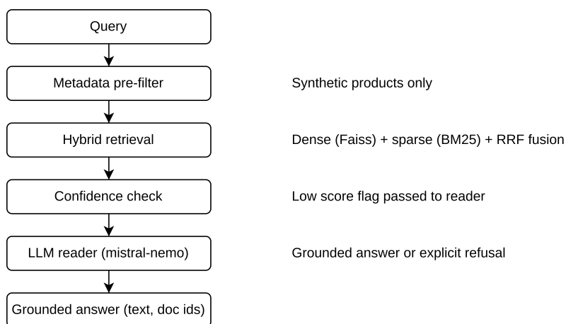
Figure 1: System workflow.
