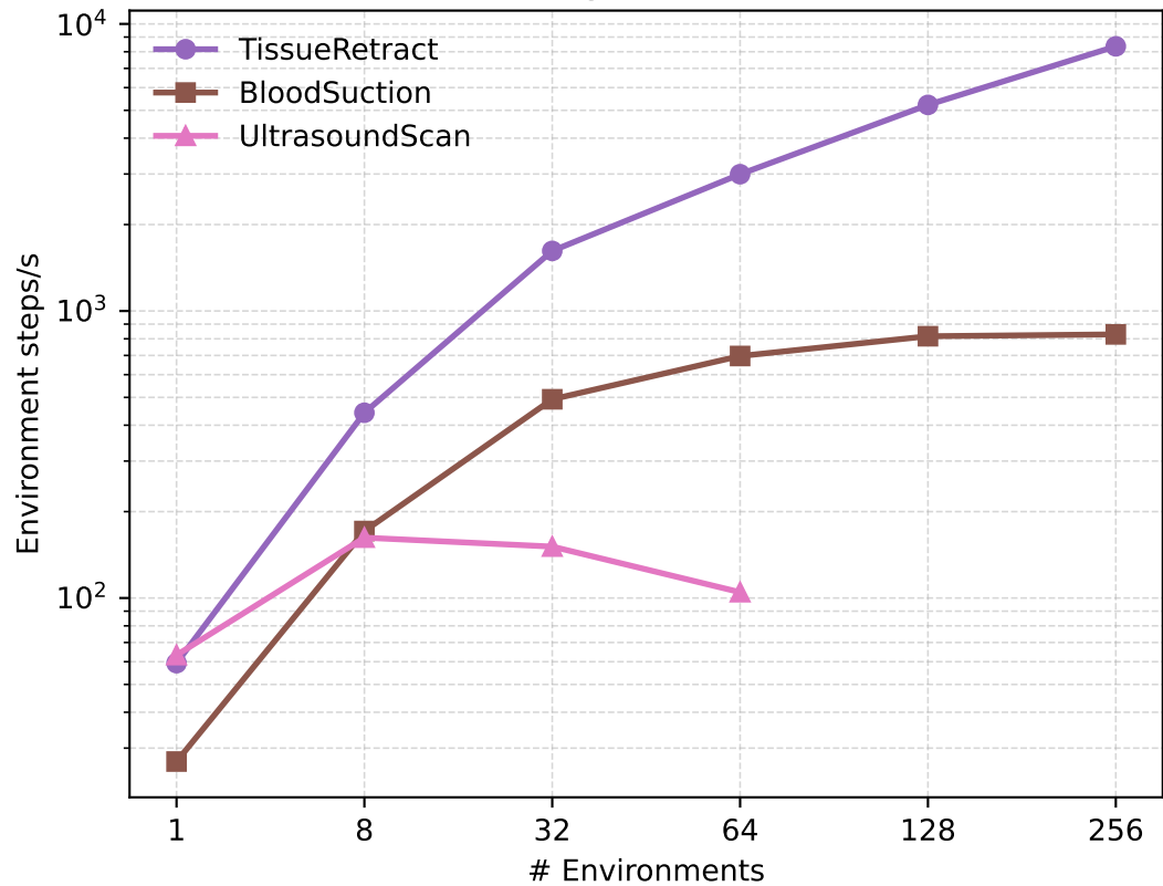
Surgical Tasks
