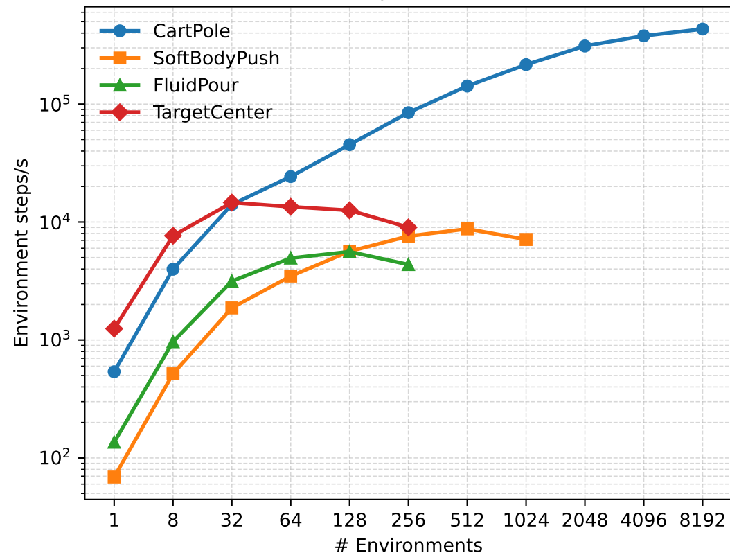
Simple Tasks
