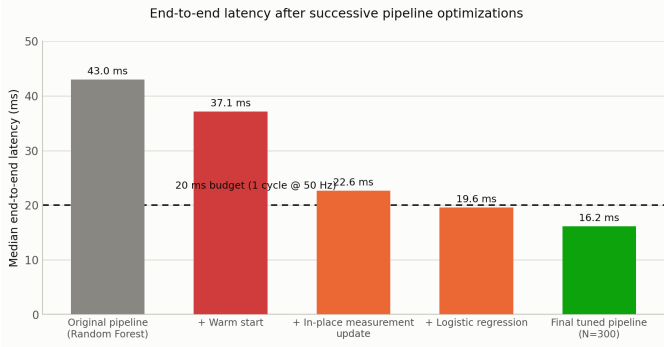
Fig. 2. End-to-end latency after successive pipeline optimizations. In-place measurement updates account for most of the reduction; the lighter classifier provides a smaller additional improvement.
