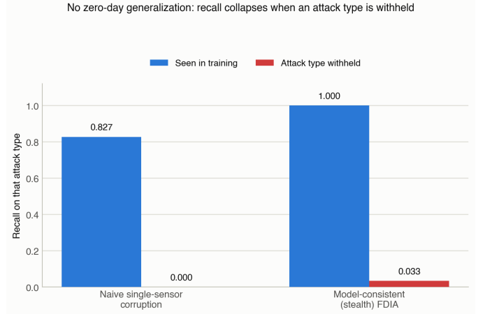
Fig. 3. Recall collapses when an attack type is withheld from training ( topology_fusion shown; residual_plus_prior is behaviorally identical, Table II).
