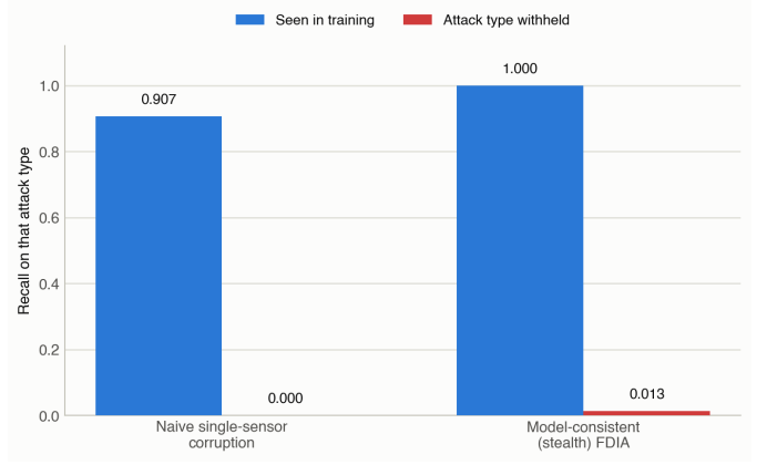
Fig. 3. Recall for attack types represented in training versus withheld from training (topology fusion shown; residual+prior is behaviorally identical, Table II).
