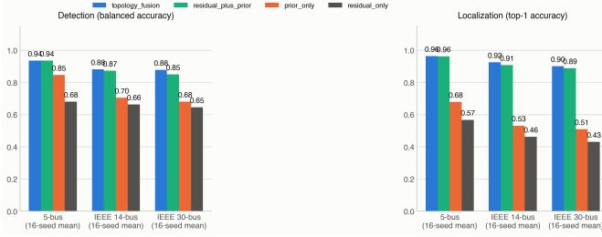
Fig. 4. 5-bus vs. IEEE 14-bus vs. IEEE 30-bus, all 16-seed means, all four feature sets. The gap is network-specific, not task-specific: null on both tasks at 5-bus, a small but mostly statistically confirmed advantage on both tasks at IEEE 14-bus and IEEE 30-bus (Table IV).
