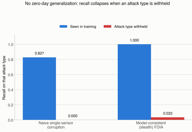
Fig. 3. Recall collapses when an attack type is withheld from training ( topology_fusion shown; residual_plus_prior is behaviorally identical, Table II).
