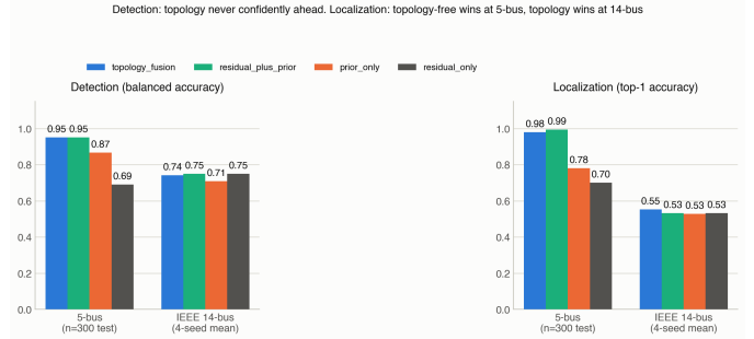
Fig. 4. 5-bus vs. IEEE 14-bus (14-bus: 4-seed mean), all four feature sets at both scales. Detection: topology_fusion never confidently ahead, at either scale. Localization: the topology-free ablation wins decisively at 5-bus; topology_fusion keeps a small, seed-robust lead at 14-bus (Table IV) – the one reversal in this paper.
