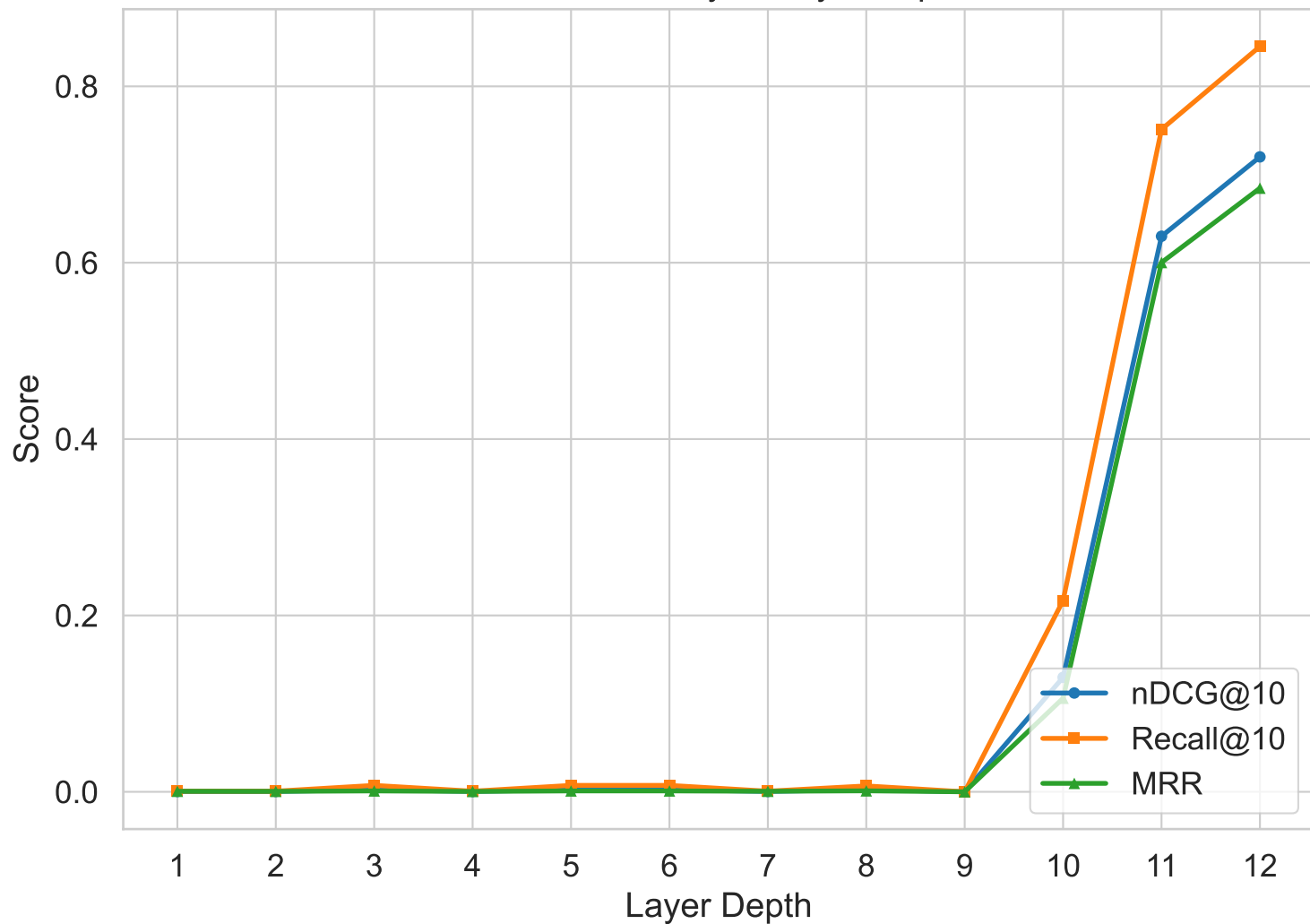
Retrieval Quality vs Layer Depth
