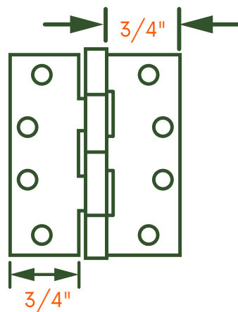
Narrow (NRW)
