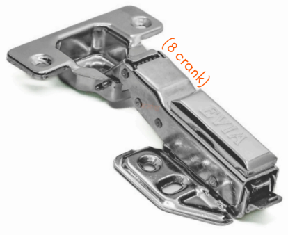
8 (Half Overlay).
