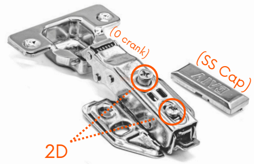
0 (Full Overlay).
