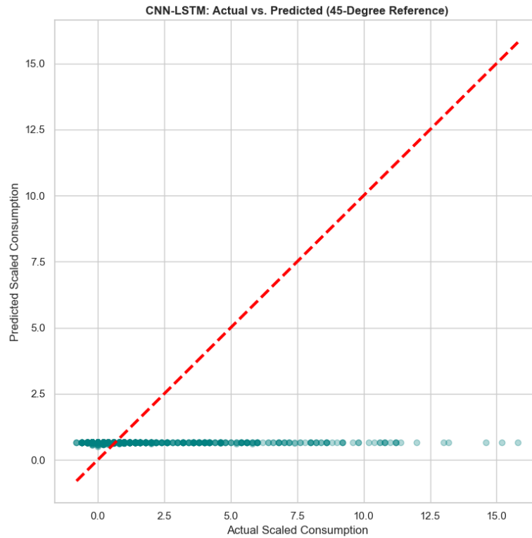
Figure 6.3: Actual vs. Predicted 45-degree scatter reference. The horizontal clustering of the CNN-LSTM predictions reveals a systematic failure to predict high-consumption events.
