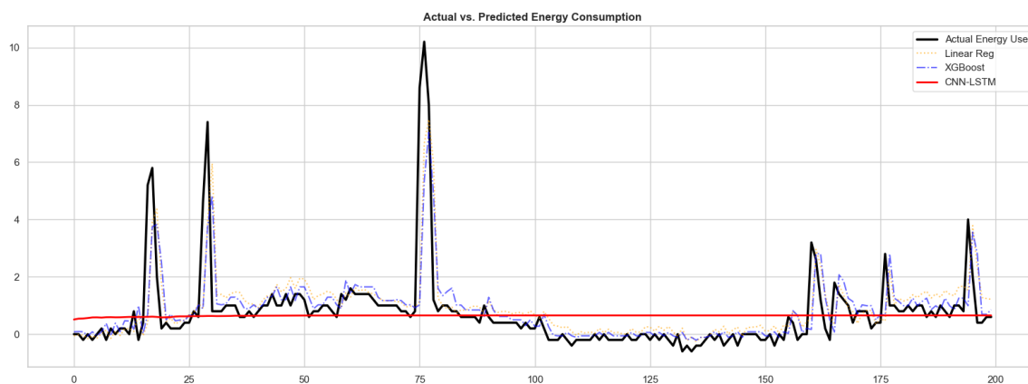
Figure 6.2: Time-series prediction tracking. Note how XGBoost aggressively and successfully maps the extreme energy spikes, while the CNN-LSTM suffers from mean-collapse, predicting a flat baseline.
