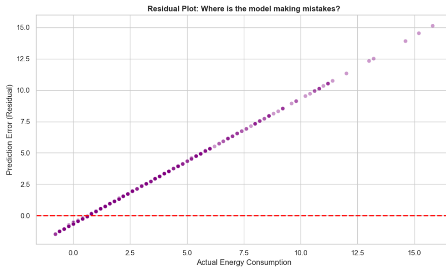
Figure 6.4: Residual scatter plot. The perfect diagonal trajectory indicates that as actual energy consumption scales up, the model's predictive error scales at a 1:1 ratio, proving it is entirely blind to peak anomalies.
