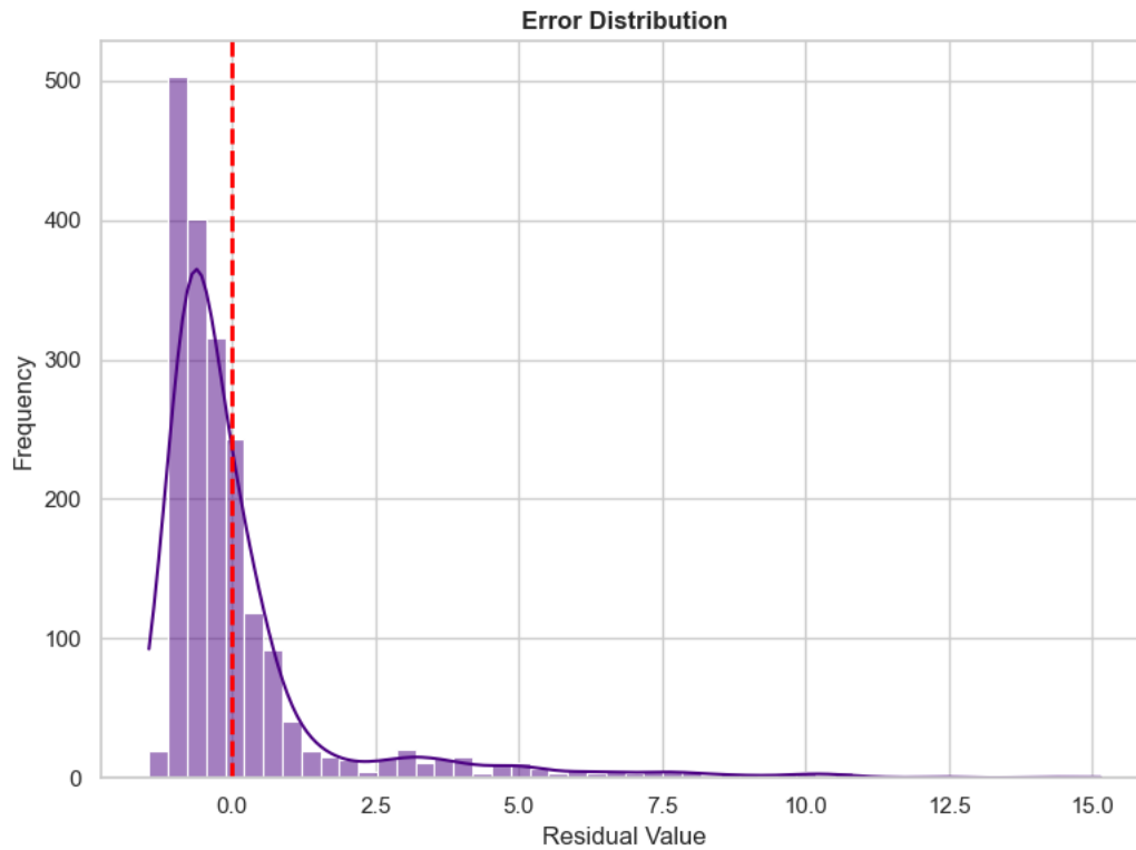
Figure 6.5: Error distribution. The pronounced right-skew and heavy tail extending toward 15 visually quantifies the CNN-LSTM's systematic underprediction of extreme load events. Rather than an optimal Gaussian spread, this skew highlights the model's conservative bias during peak anomalies.
