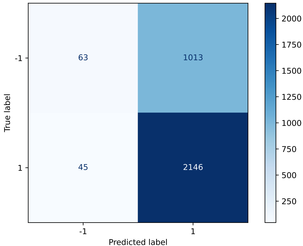
Confusion Matrix ( \alpha = 0.8 )
