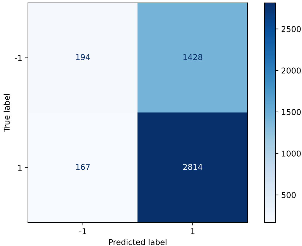
Confusion Matrix ( \alpha = 0.6 )
