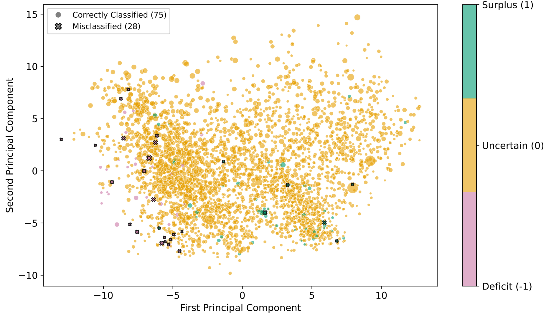
Decision Boundary in PCA Space ( \alpha = 0.80 , Accuracy=72.8%)
