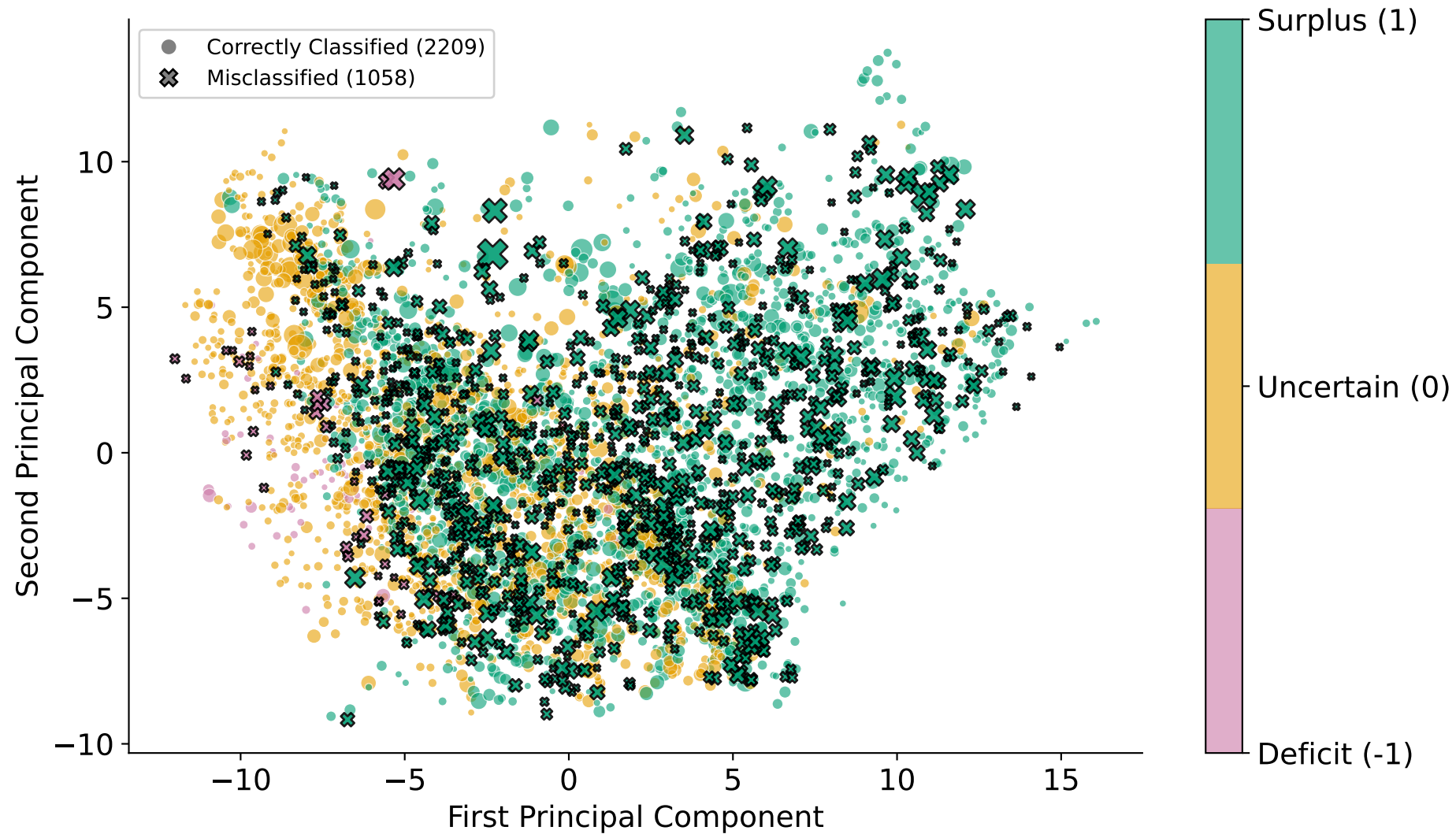
Decision Boundary in PCA Space ( \alpha = 0.80 , Accuracy=67.6%)
