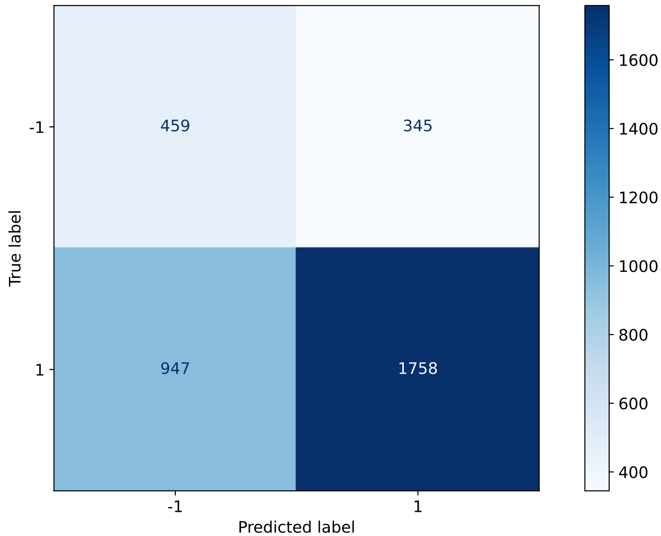
Confusion Matrix ( \alpha = 0.5 )
