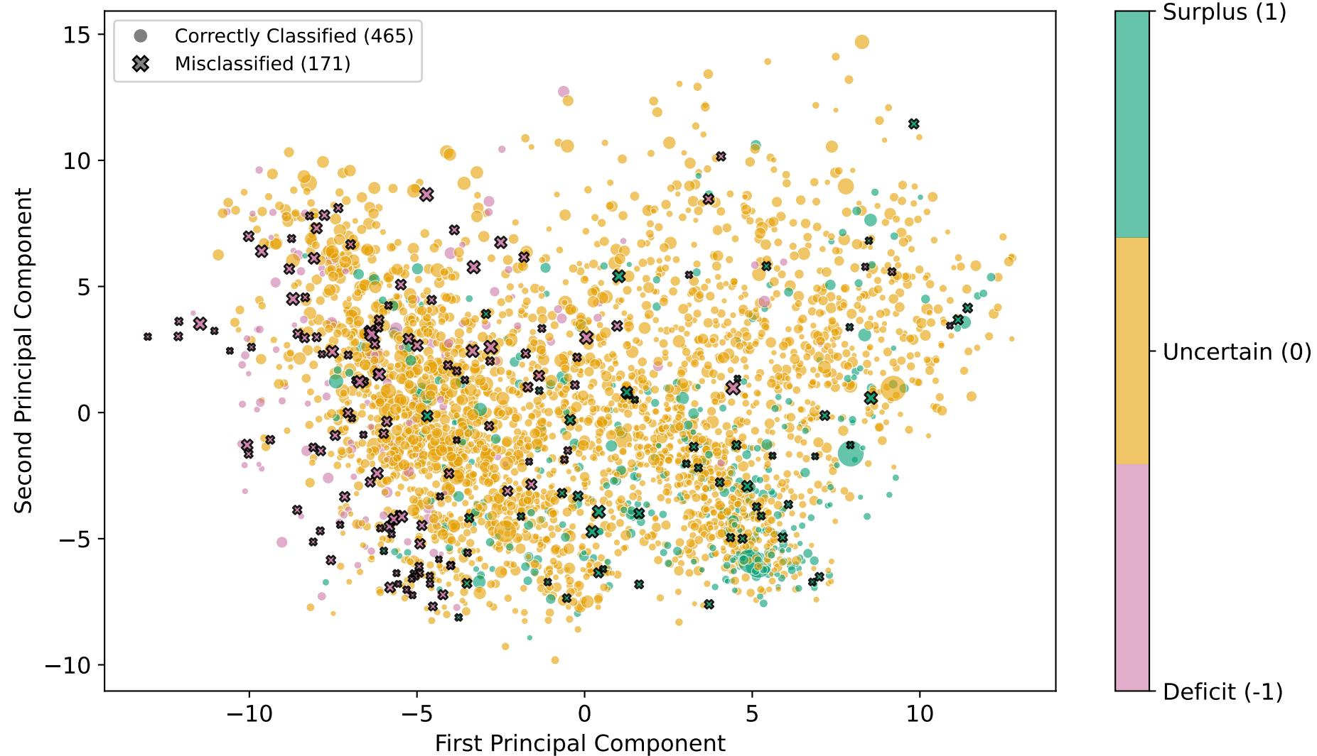
Decision Boundary in PCA Space ( \alpha = 0.70 , Accuracy=73.1%)
