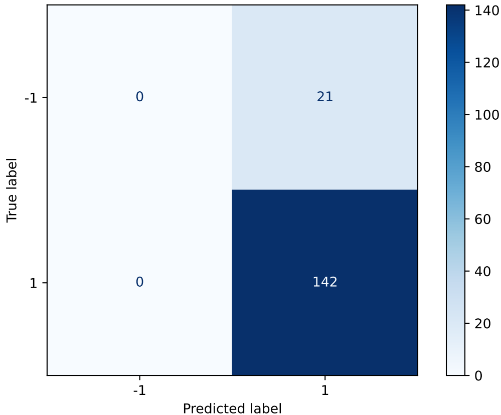
Confusion Matrix ( \alpha = 0.9 )
