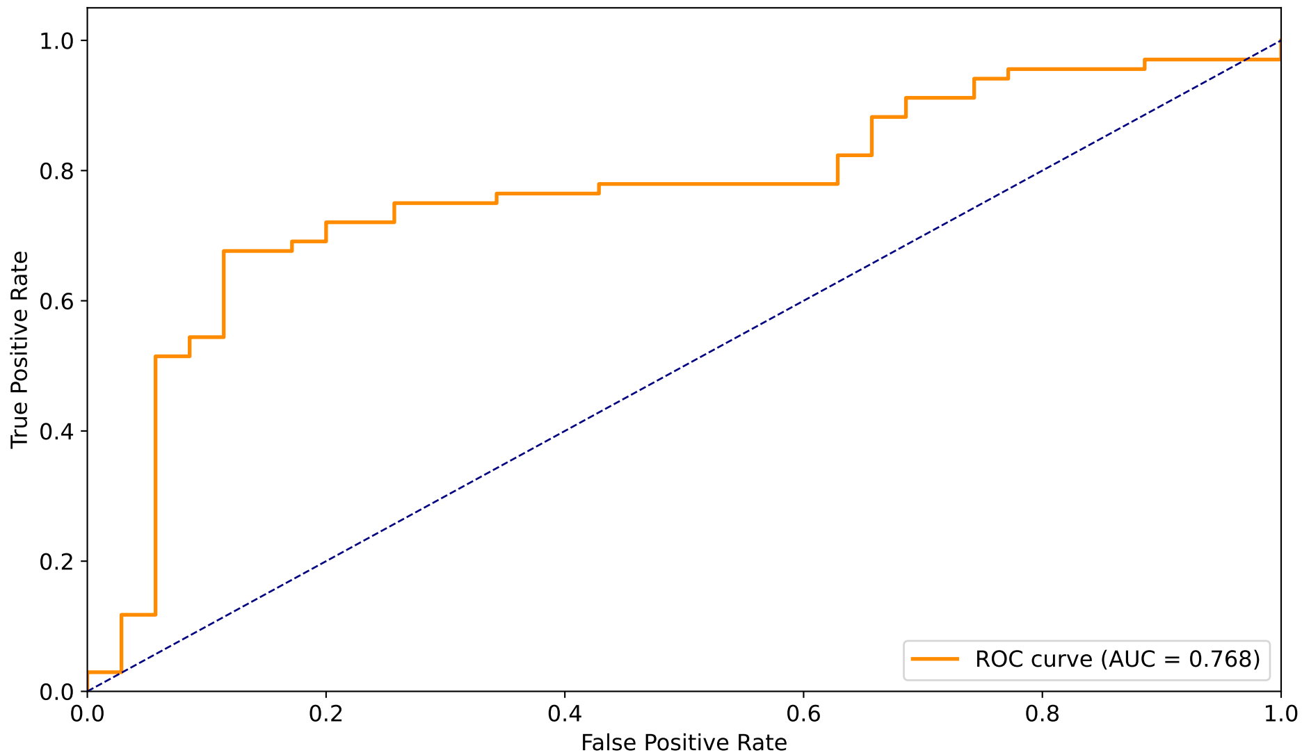
ROC Curve ( \alpha = 0.8 )
