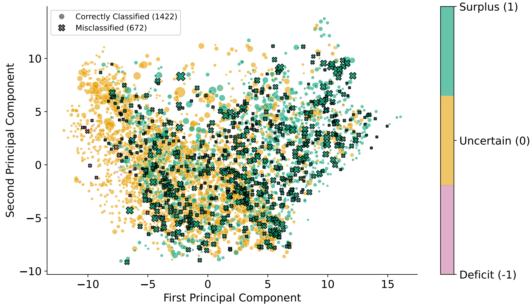
Decision Boundary in PCA Space ( \alpha = 0.90 , Accuracy=67.9%)
