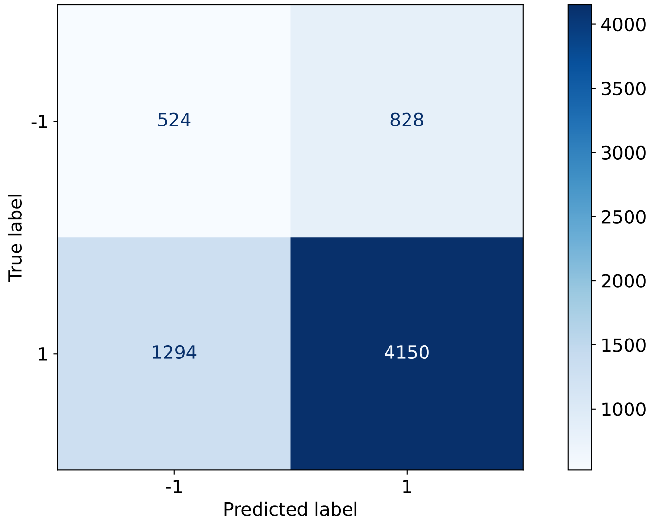
Confusion Matrix ( \alpha = 0.6 )
