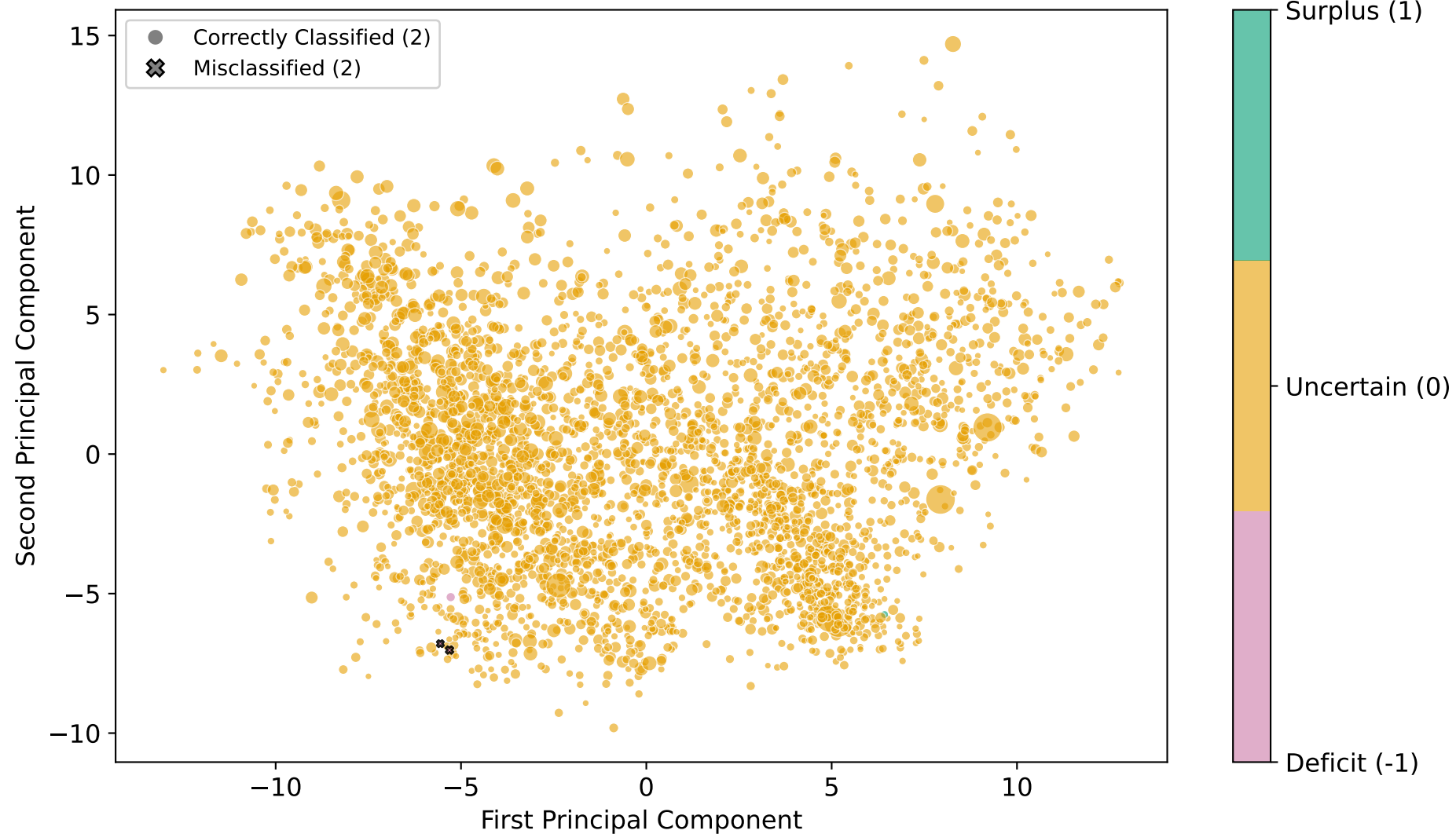
Decision Boundary in PCA Space ( \alpha = 0.90 , Accuracy=50.0%)
