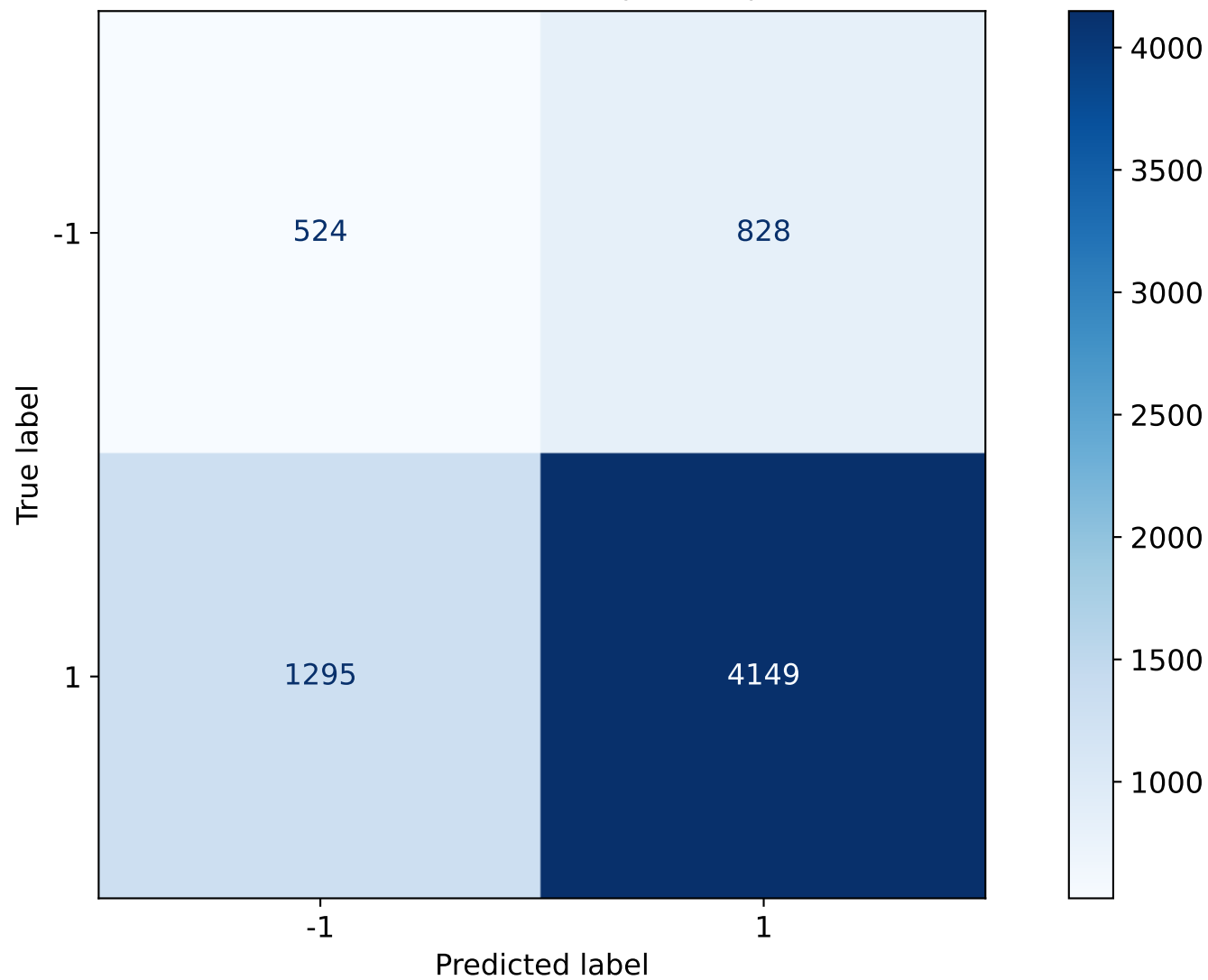
Confusion Matrix ( \alpha = 0.6 )
