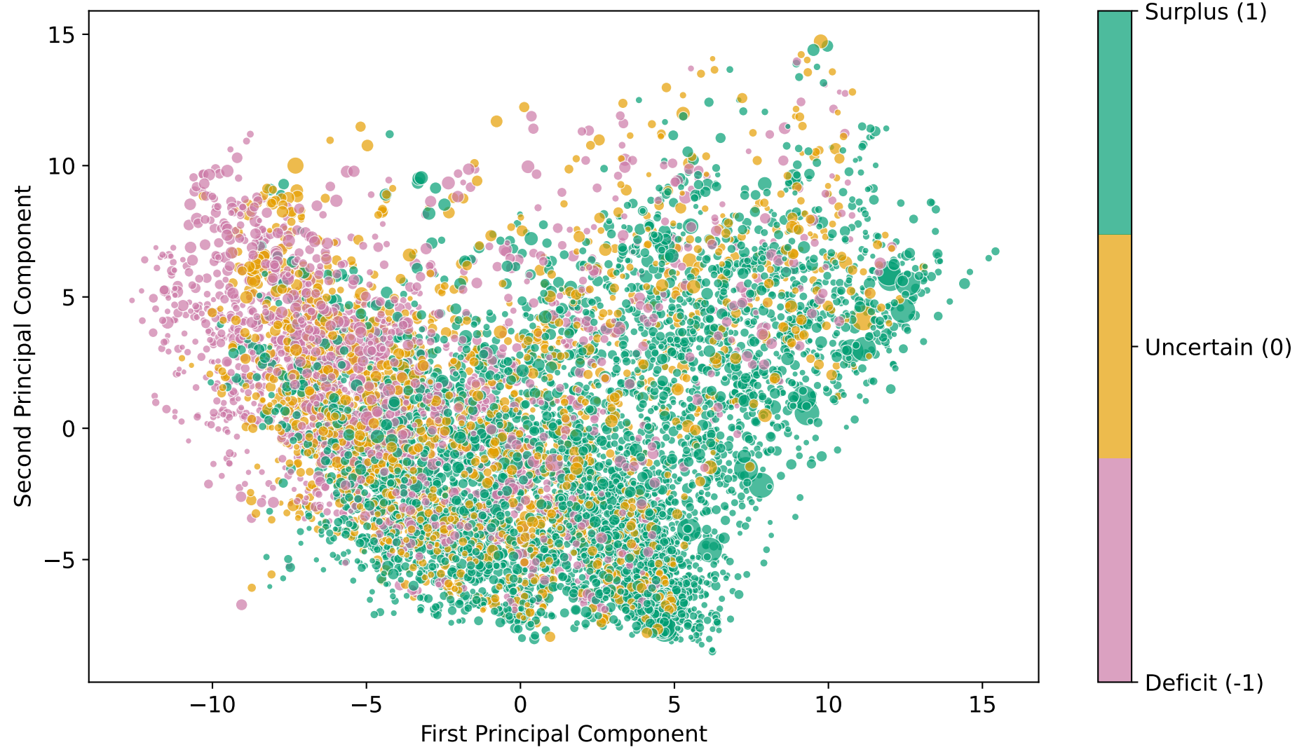
Decision Boundary in PCA Space ( \alpha = 0.60 , Accuracy=68.8%)
