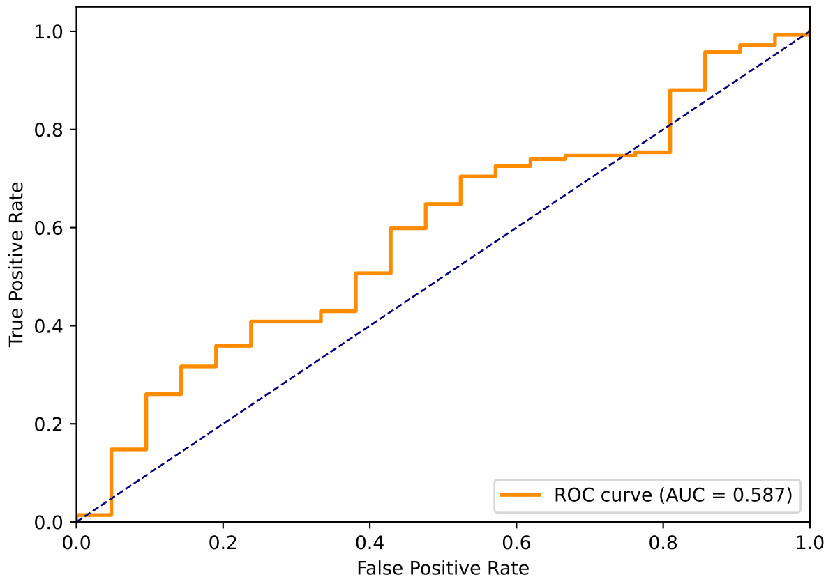
ROC Curve ( \alpha = 0.9 )
