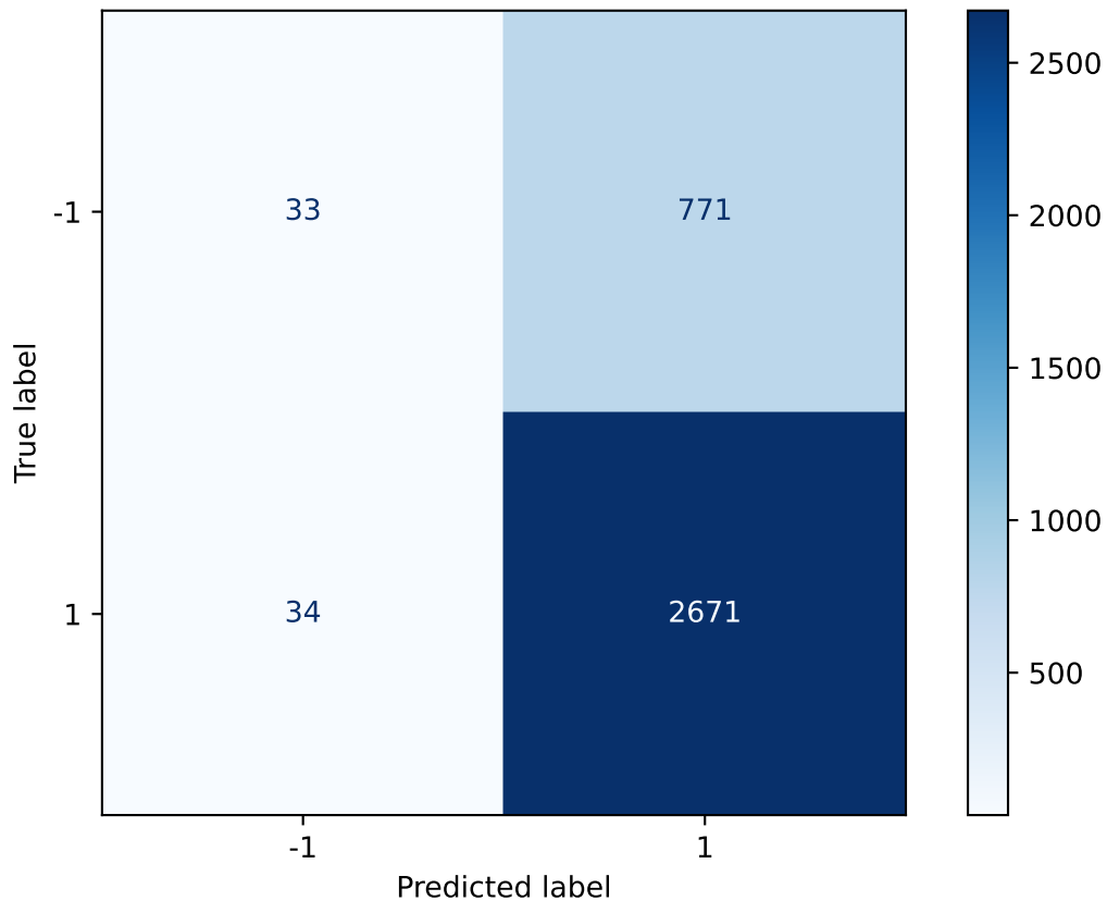
Confusion Matrix ( \alpha = 0.5 )
