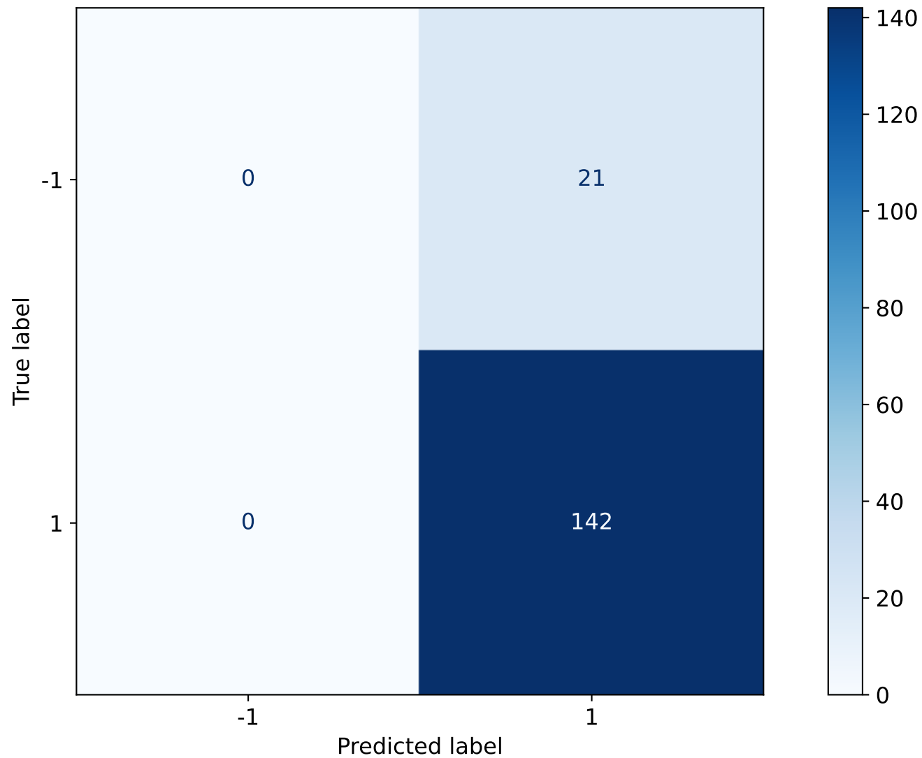
Confusion Matrix ( \alpha = 0.9 )
