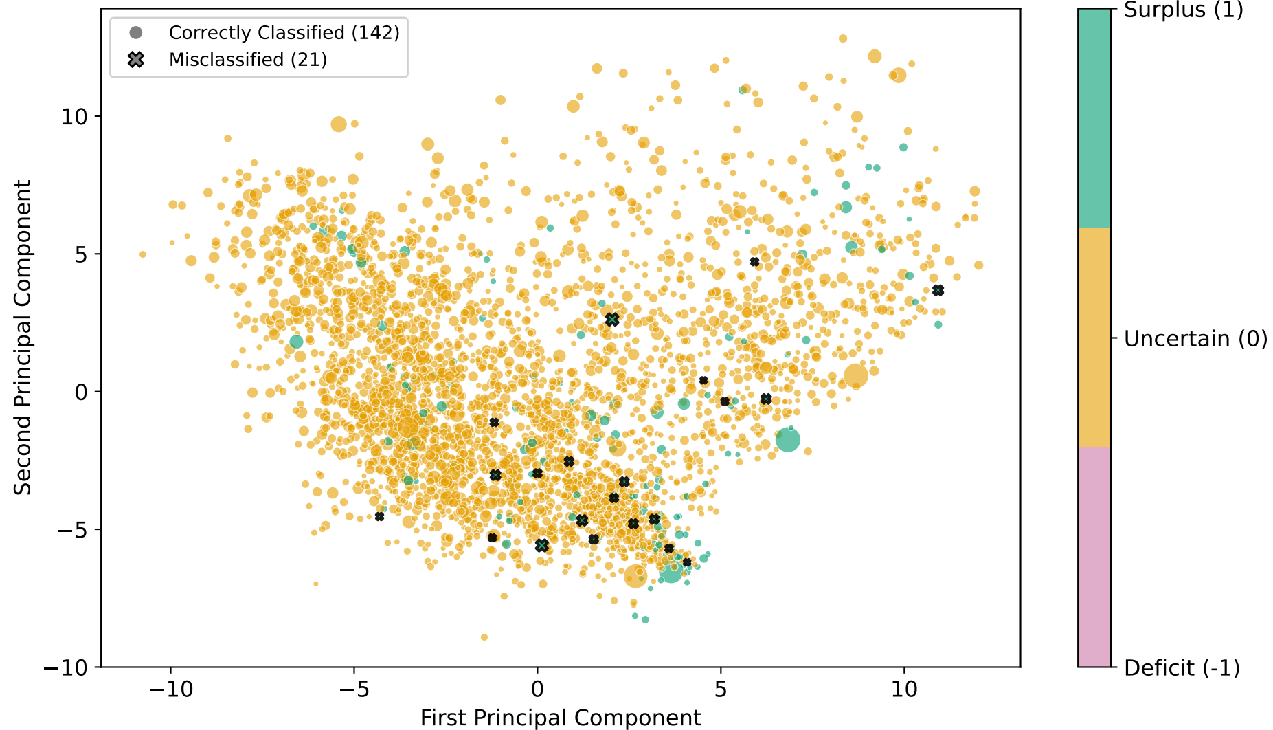
Decision Boundary in PCA Space ( \alpha = 0.90 , Accuracy=87.1%)
