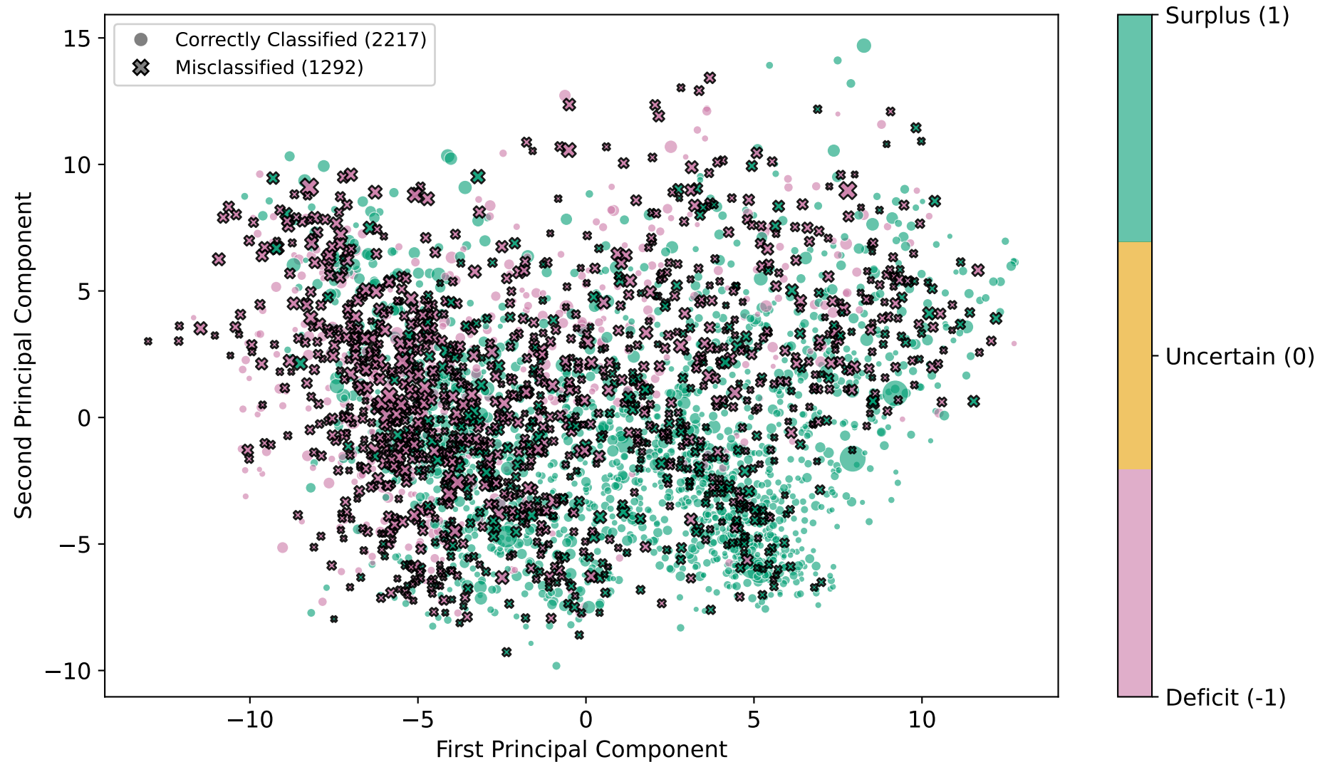
Decision Boundary in PCA Space ( \alpha = 0.50 , Accuracy=63.2%)
