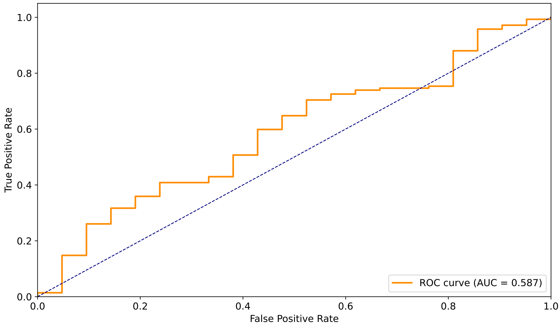
ROC Curve ( \alpha = 0.9 )
