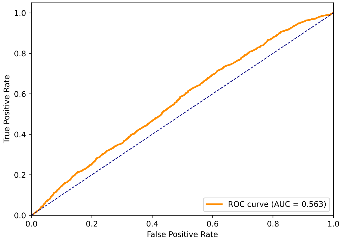
ROC Curve ( \alpha = 0.6 )
