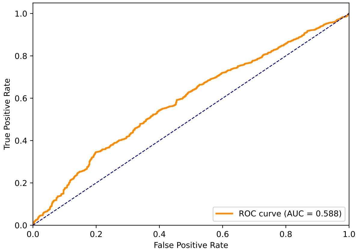
ROC Curve ( \alpha = 0.7 )
