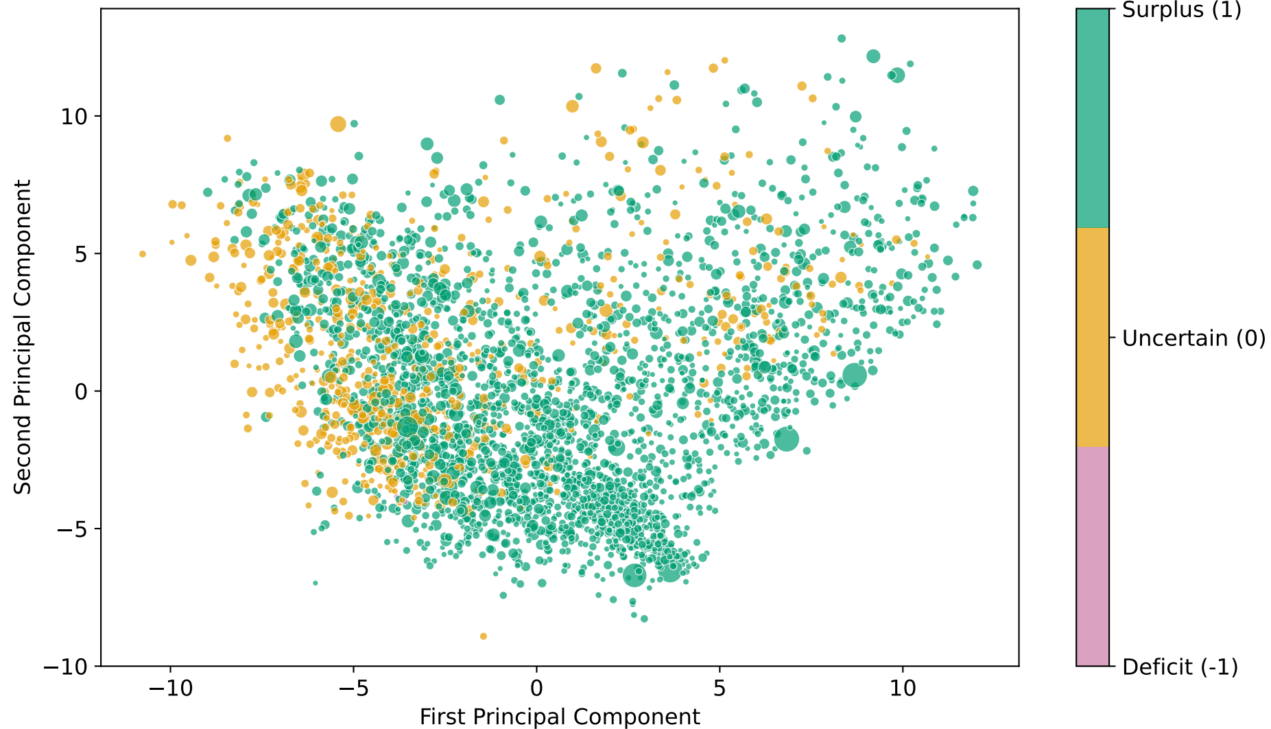
Decision Boundary in PCA Space ( \alpha = 0.70 , Accuracy=80.8%)
