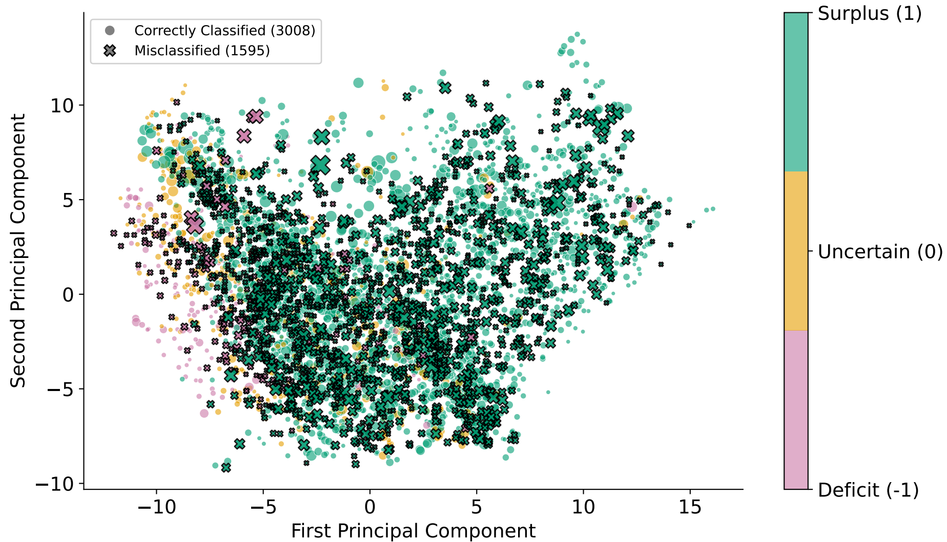
Decision Boundary in PCA Space ( \alpha = 0.60 , Accuracy=65.3%)
