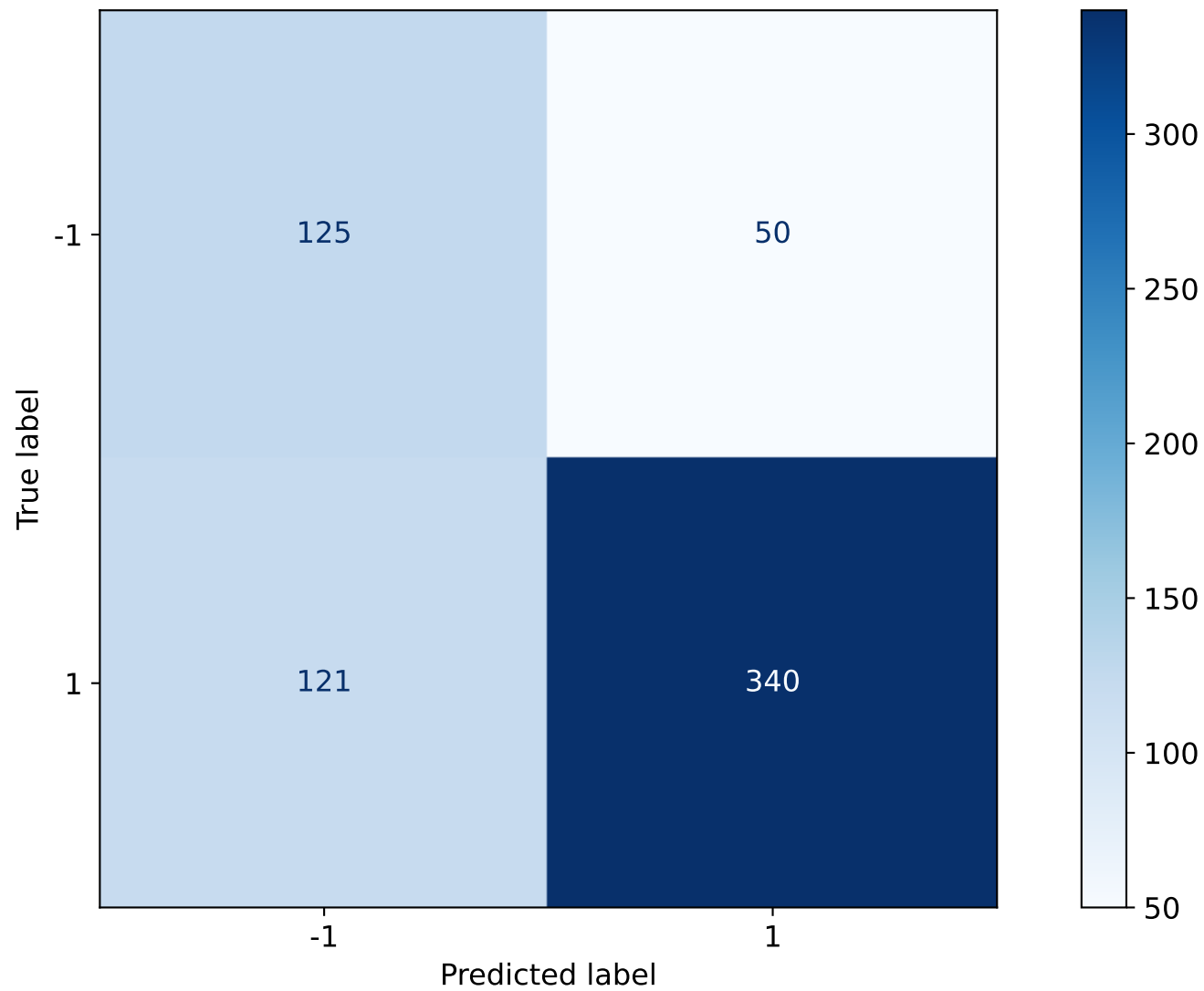
Confusion Matrix ( \alpha = 0.7 )
