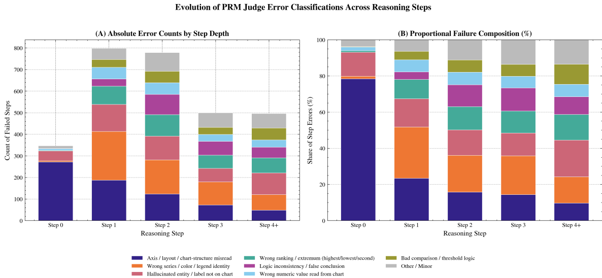
Figure 6: Error Mode Composition Across Step Depth. Detailed breakdown of 2,920 refuted reasoning steps evaluated by muse-spark-1.1 across reasoning steps 0 to 4+. Step 0 is dominated by axis and layout misreads (78.5%), which triggers cascading entity hallucinations and logical inconsistencies in downstream steps.
