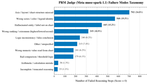
Figure 2: Distribution of 2,920 Refuted Reasoning Steps. Visual grounding failures (axis misreads at 24.0% and series confusion at 19.5%) account for 43.5% of all errors, whereas pure arithmetic mistakes account for only 1.3%.
