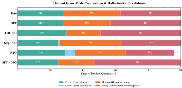
Figure 8: Holdout Error Mode Breakdown. Partitioning of test responses into extracted correct, unextracted correct in prose, partial ground-truth mentions, and committed wrong answers (hallucination proxy).
