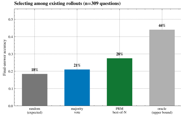
Figure 7: Inference-Time PRM Verifier Accuracy. Average step process reward selection (27.5%) outperforms self-consistency majority voting (21.0%) and random rollouts (18.4%) across 309 multi-candidate questions.
