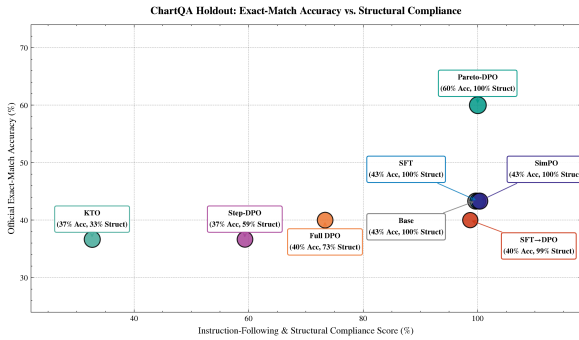
Figure 5: ChartQA Accuracy vs. Structure Trade-Off . Compare with Figure 3: on CharXiv, the trade-off separates methods along a frontier: on ChartQA, Pareto-DPO dominates outright, decisively ahead on accuracy while matching the highest structure score.
