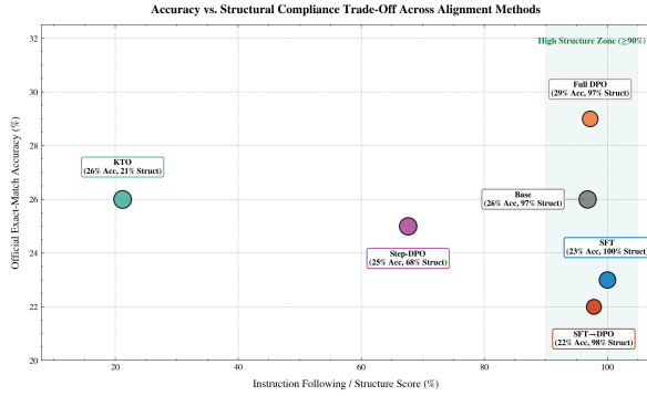
Figure 3: Accuracy vs. Structure Pareto Frontier. Bubble diameter is proportional to ground-truth mention recall in prose (47%–66%). Full DPO achieves the best balance (29.0% accuracy, 97.2% structure). SFT attains 100% structure at lower accuracy (23.0%). KTO yields highest latent recall (66.0%) but collapses structurally (21.2%).
