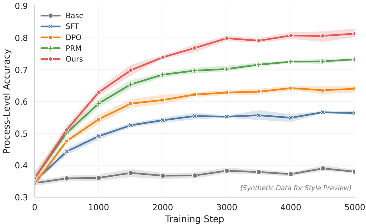
Training Step vs. Process-Level Accuracy
