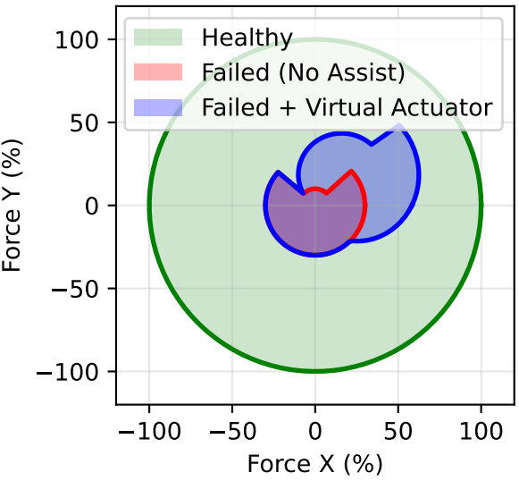
Control Authority Envelope (95% Thruster Failure)
