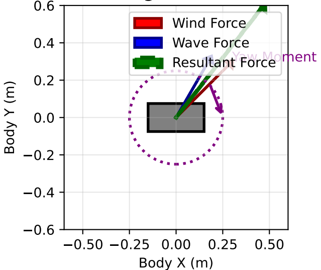
Environmental Forces on USV (15° Force Misalignment → Yaw Moment)
