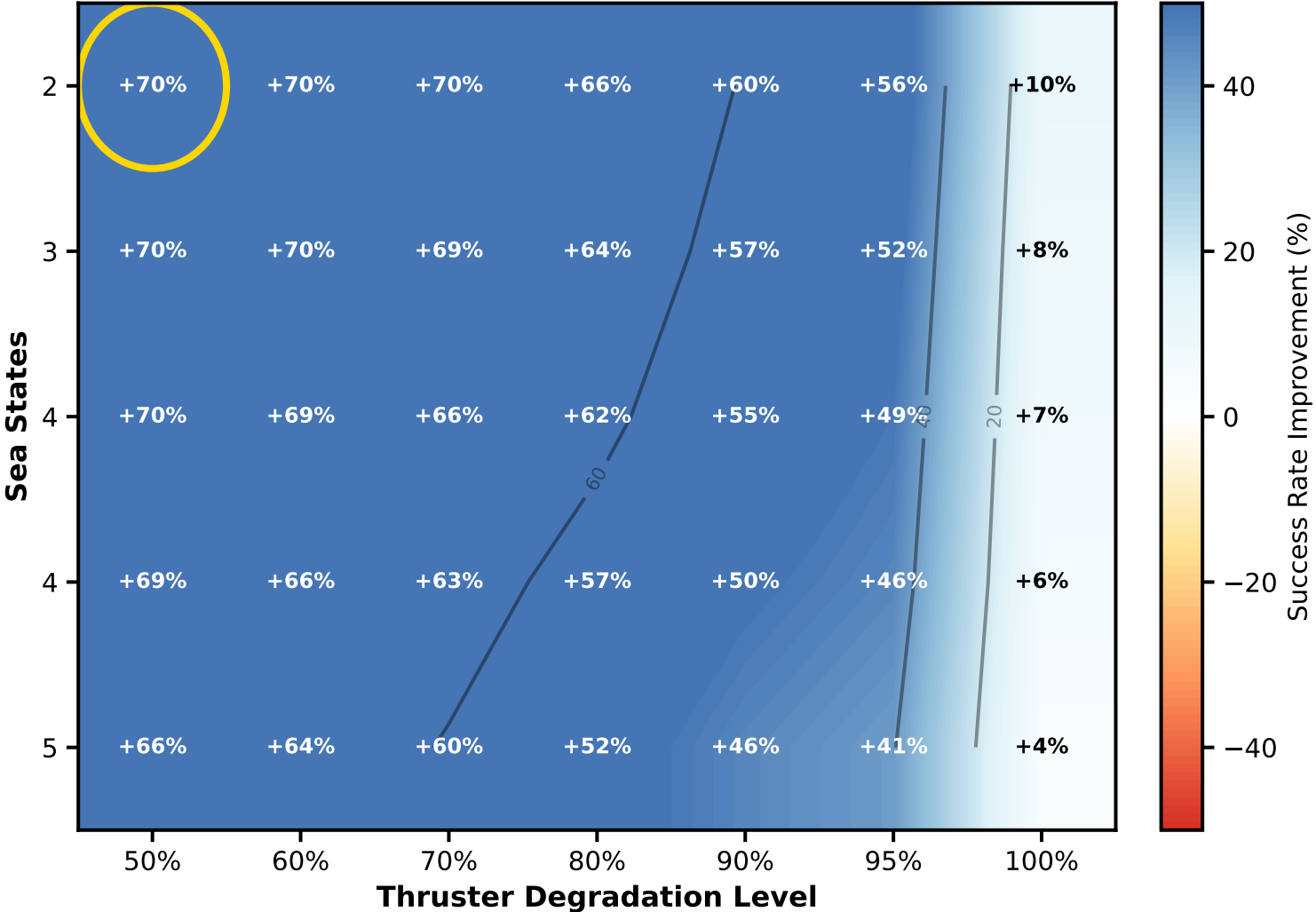
Performance Improvement: Environment-Assisted vs Baseline MPC
