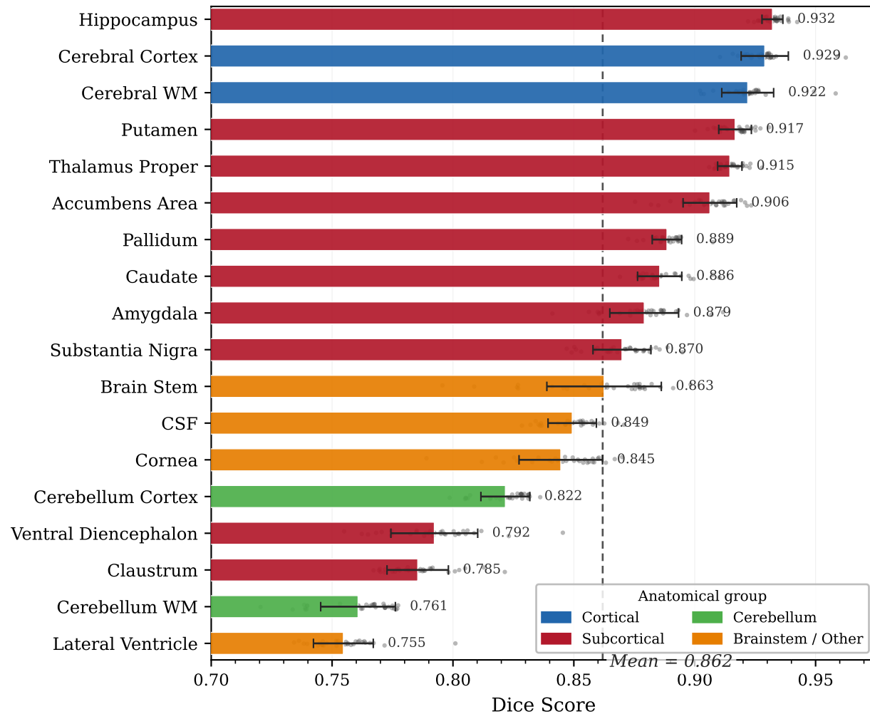
A Per-class Dice Score
