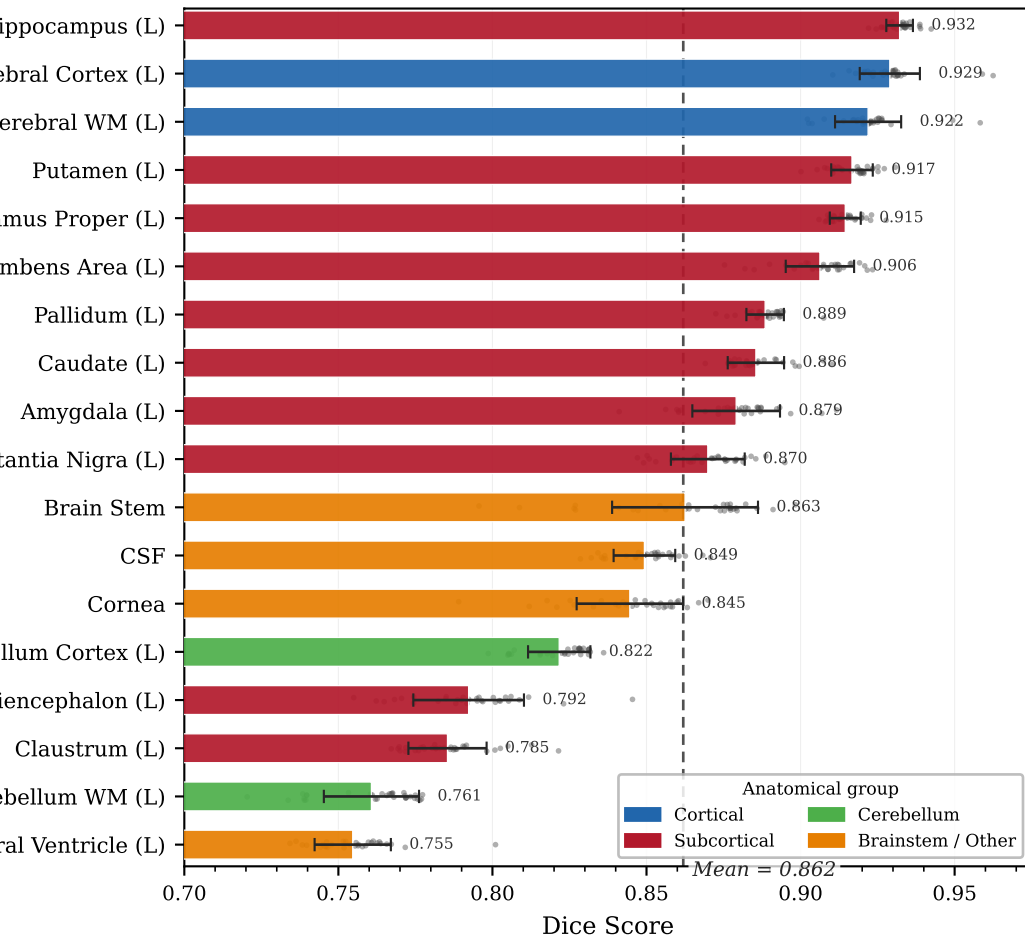
A Per-class Dice Score
