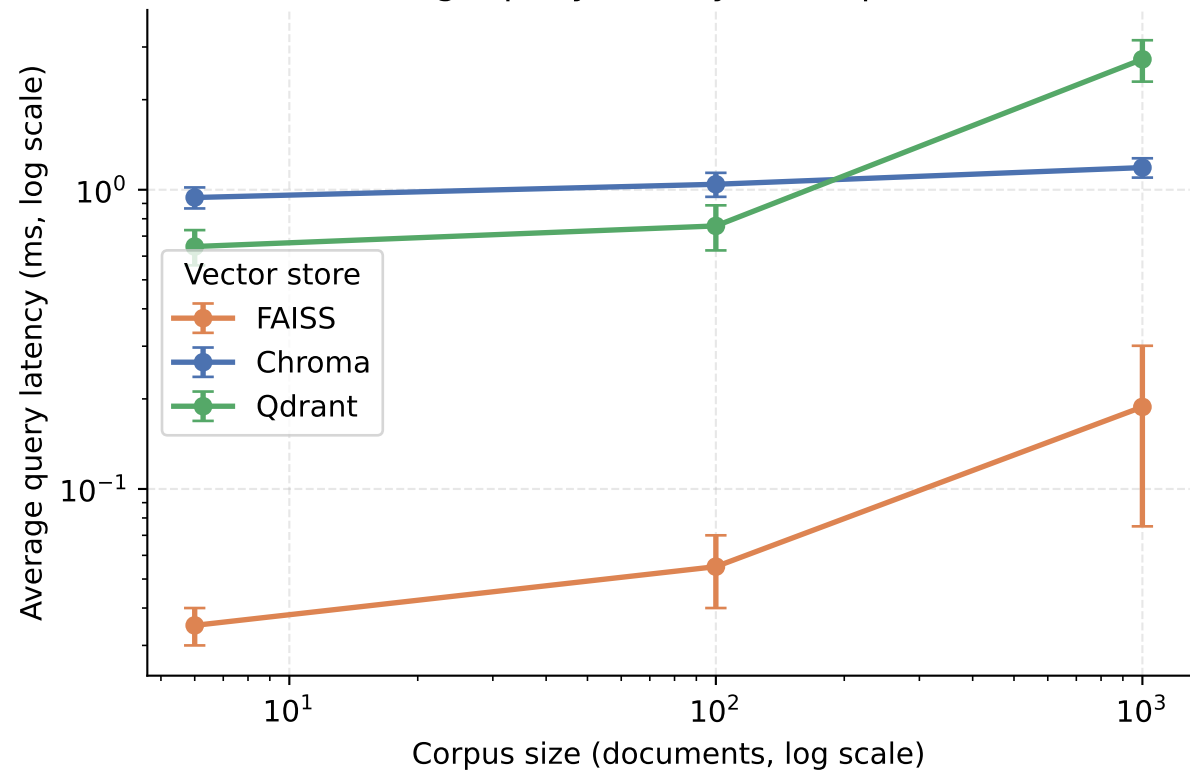
Average query latency vs. corpus size
