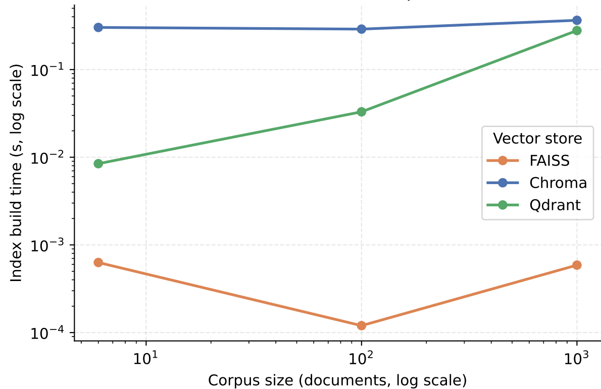
Index build time vs. corpus size
