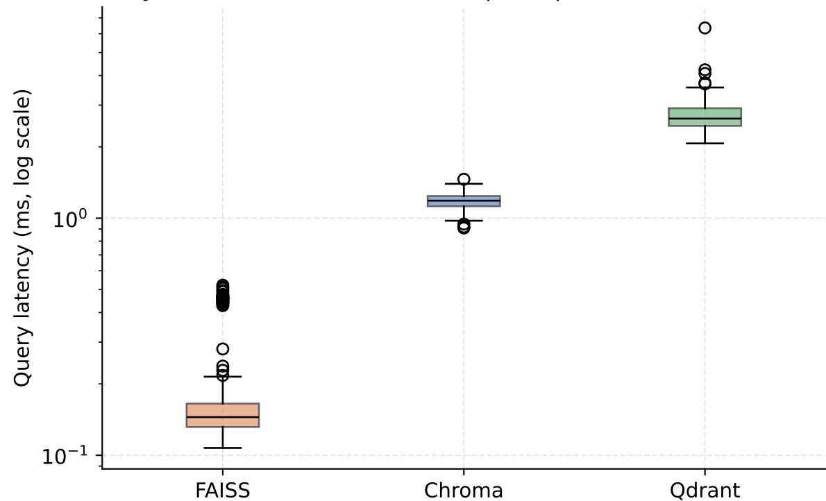
Latency distribution across all sampled queries (1000 documents)
