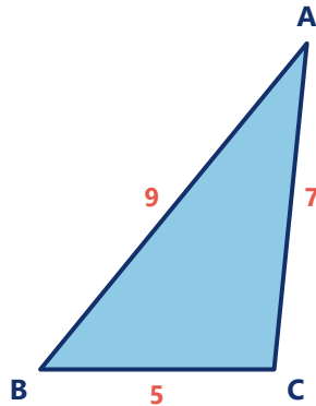
משולש ABC: AB = 9, CA = 7, BC = 5
