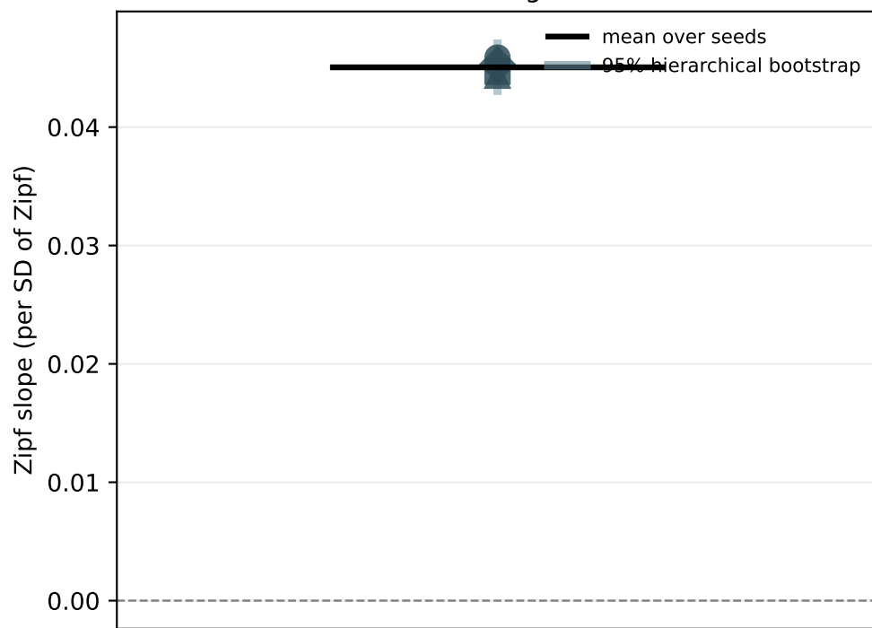
Gate g
