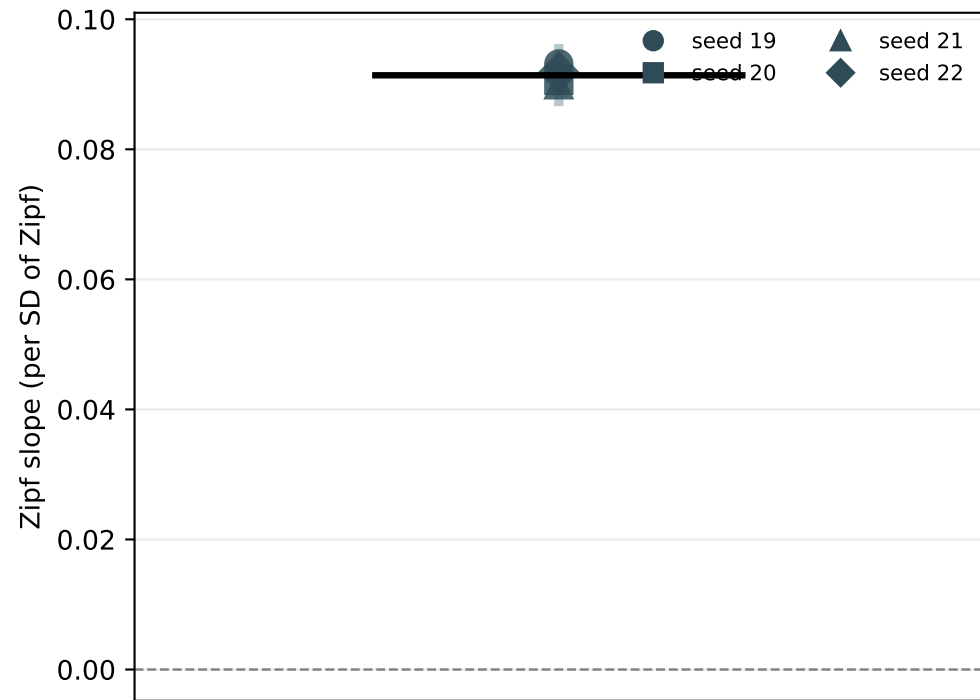
Lexical confidence
