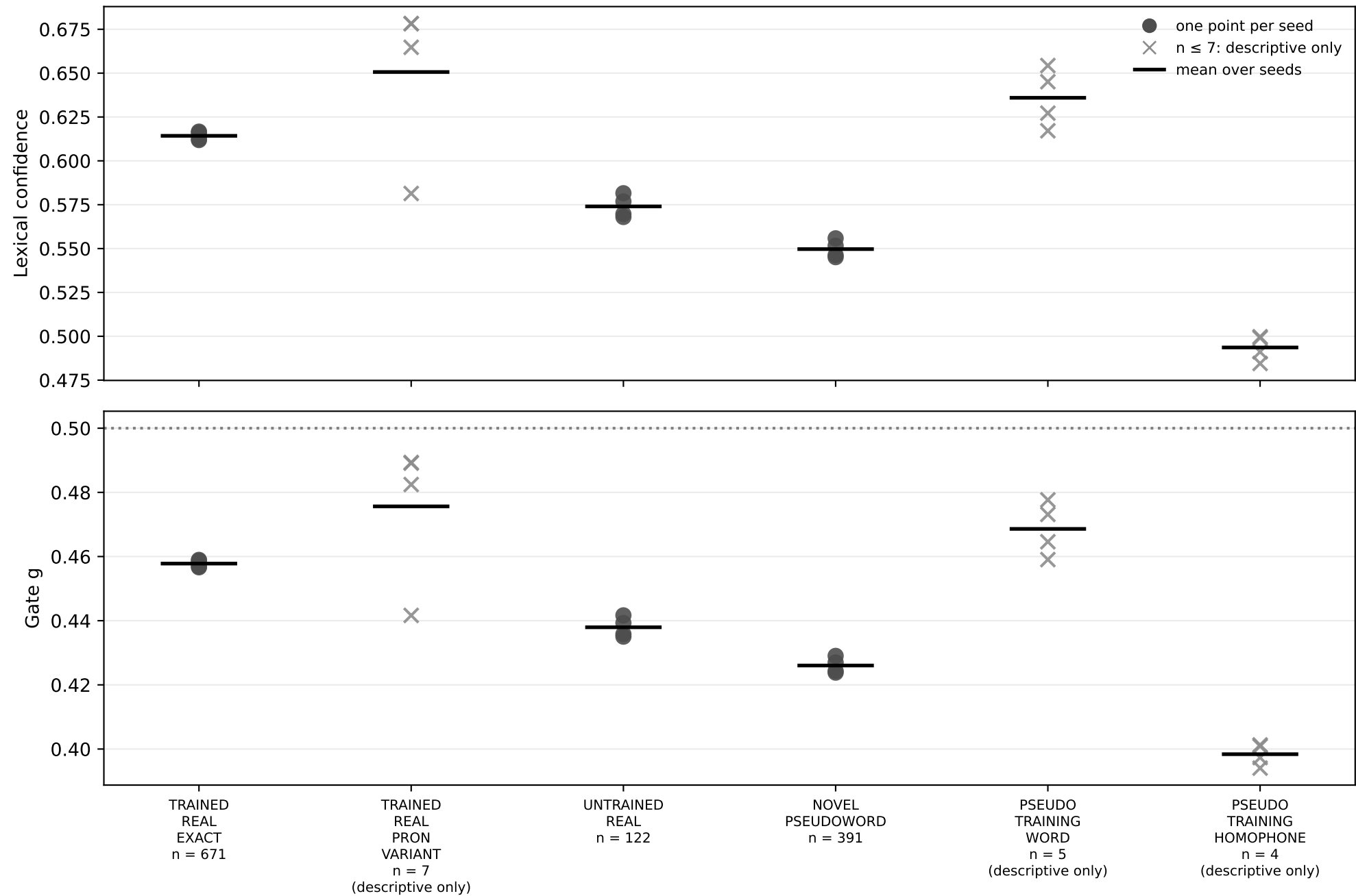
Gate and lexical confidence by training-exposure status
