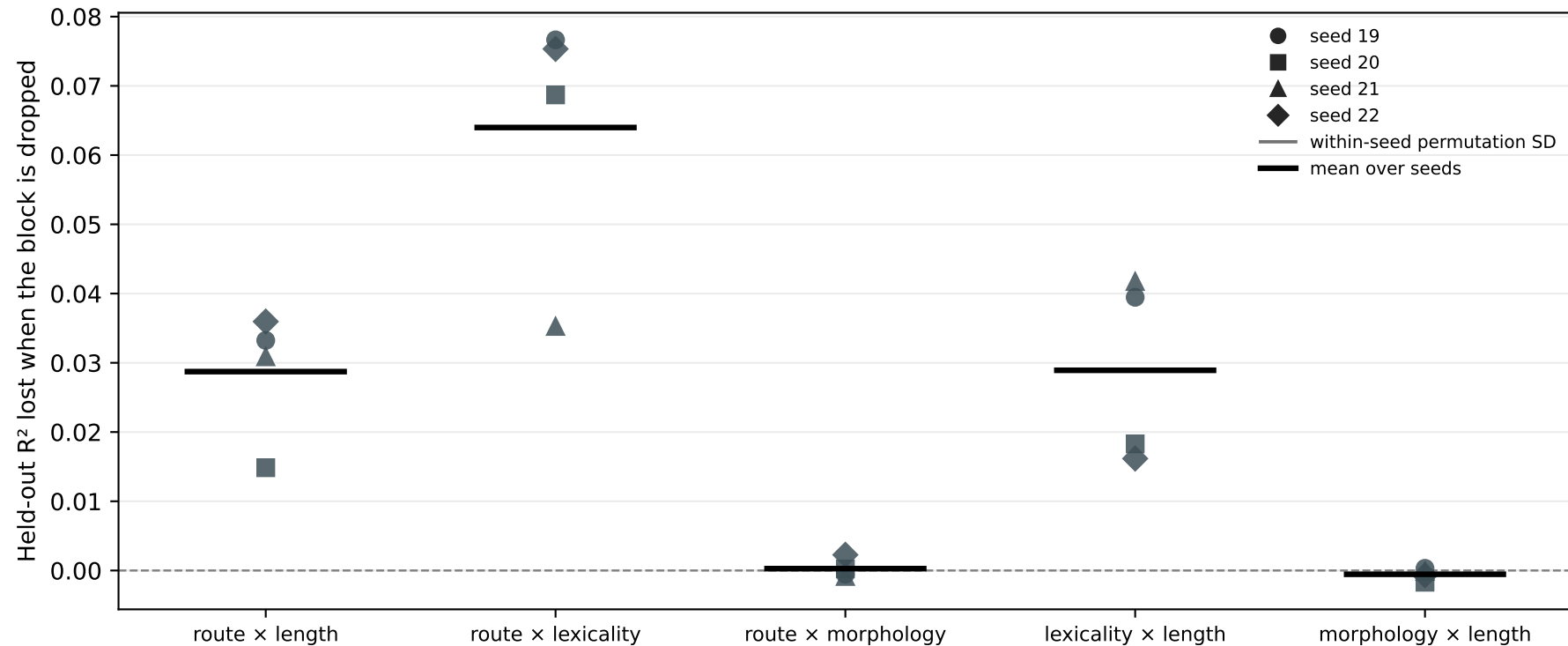
Predeclared interaction blocks — held-out drop-block utility
