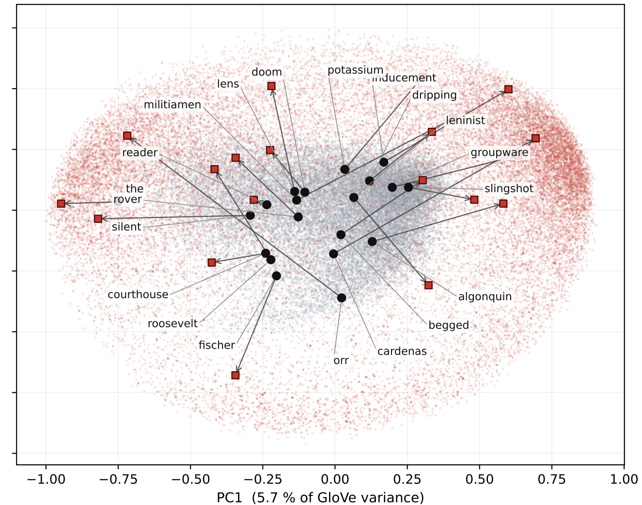
seed 22 / epoch 140
