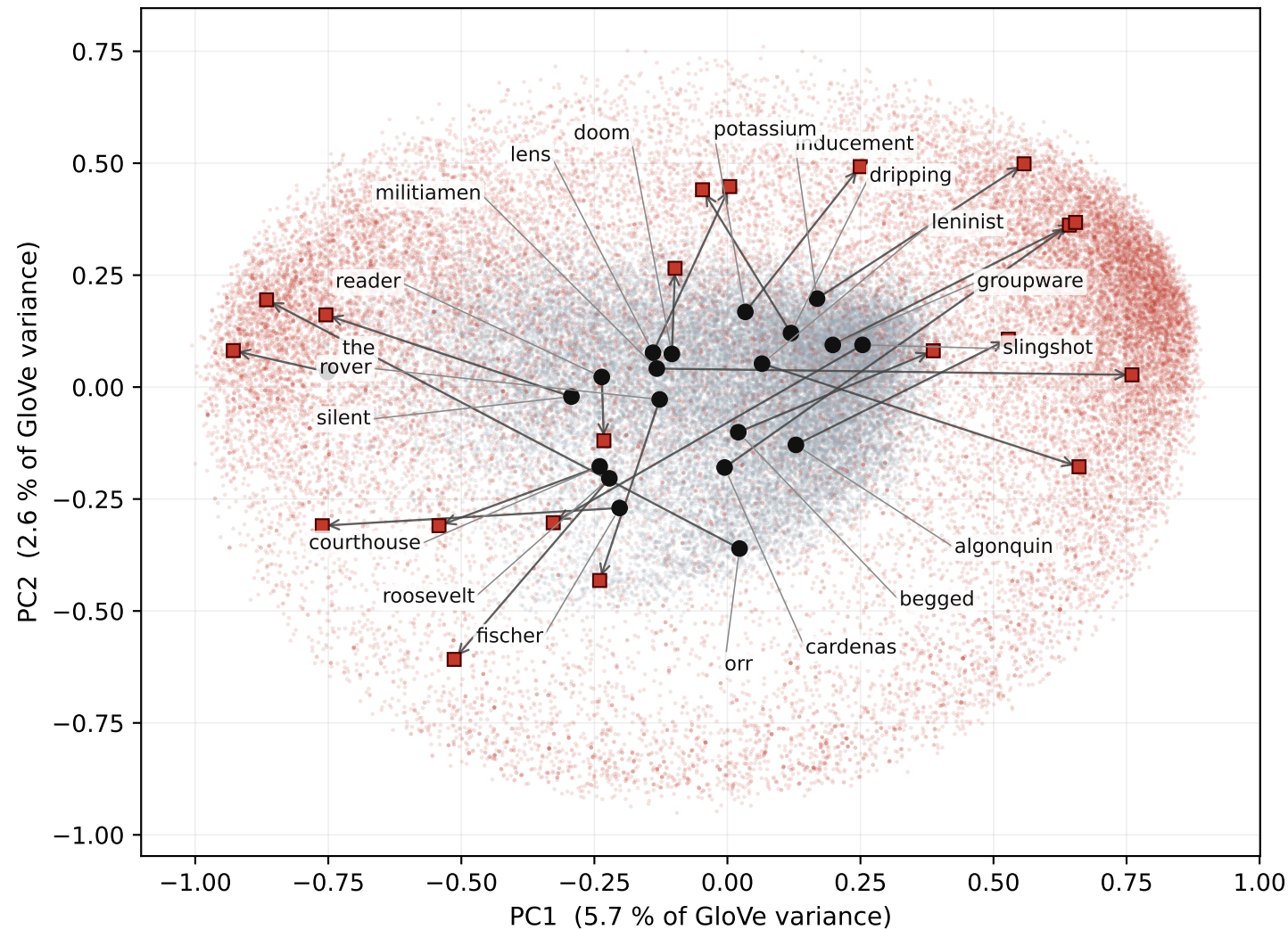
seed 19 / epoch 155
