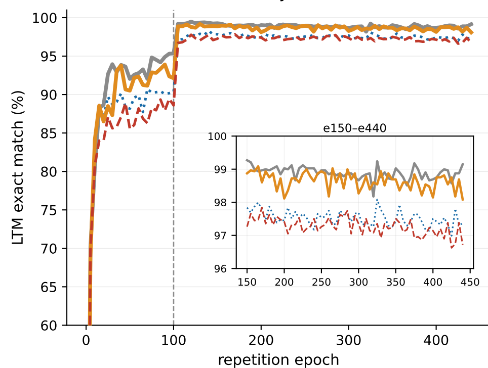
C · Isolated ventral repetition (subset3288; FULL stays \geq 99.9\% in all cells)
