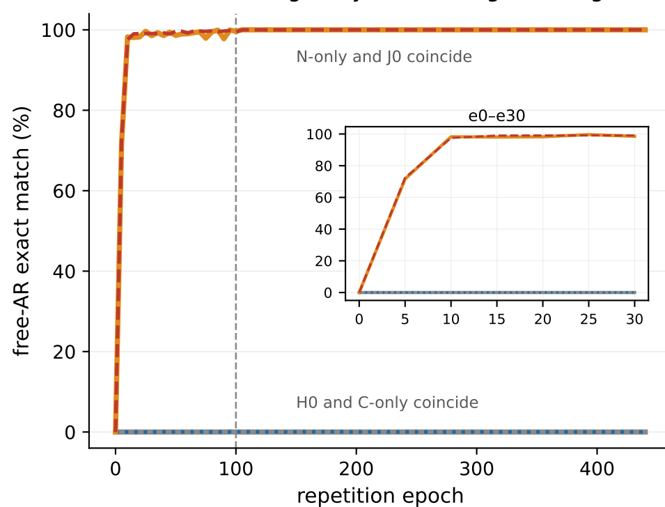
B · Naming from true GloVe (subset3288, greedy AR, no length leakage)
