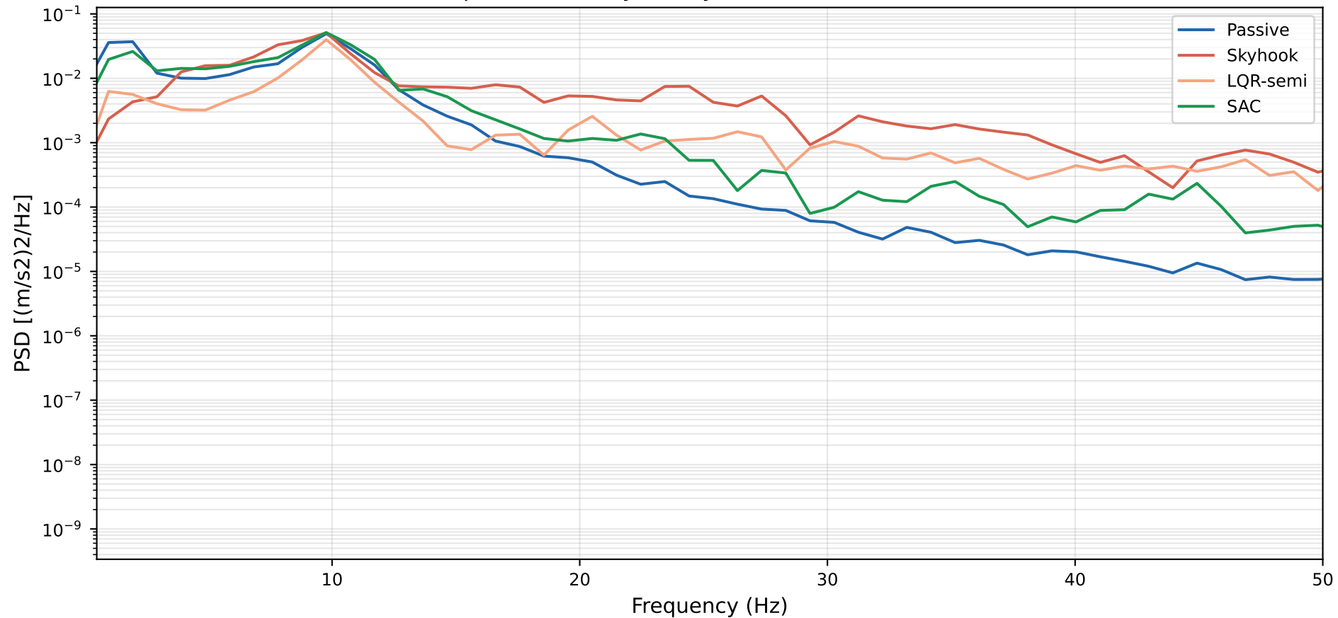
Power Spectral Density - Body Acceleration (Random Road)
