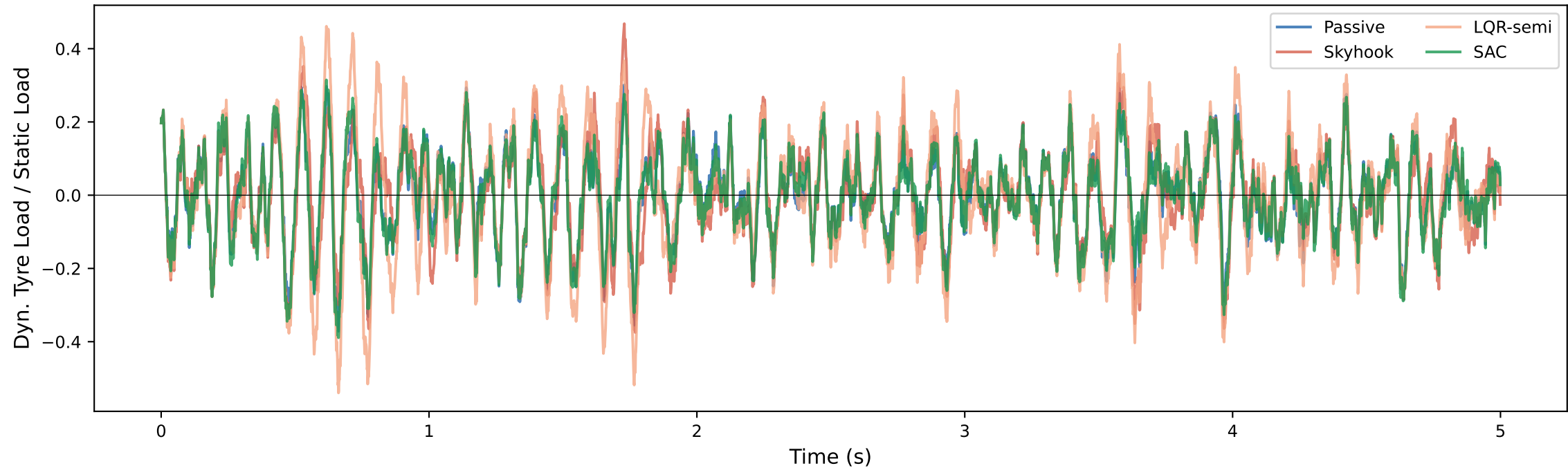
Dynamic Tyre Load - Random Road (road-holding constraint)
