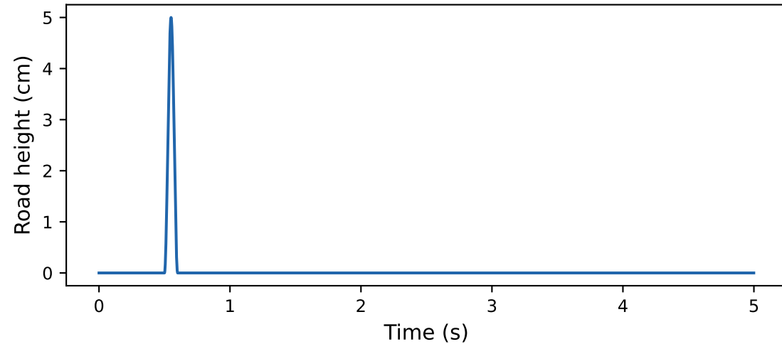
Bump Profile (5 cm haversine)
