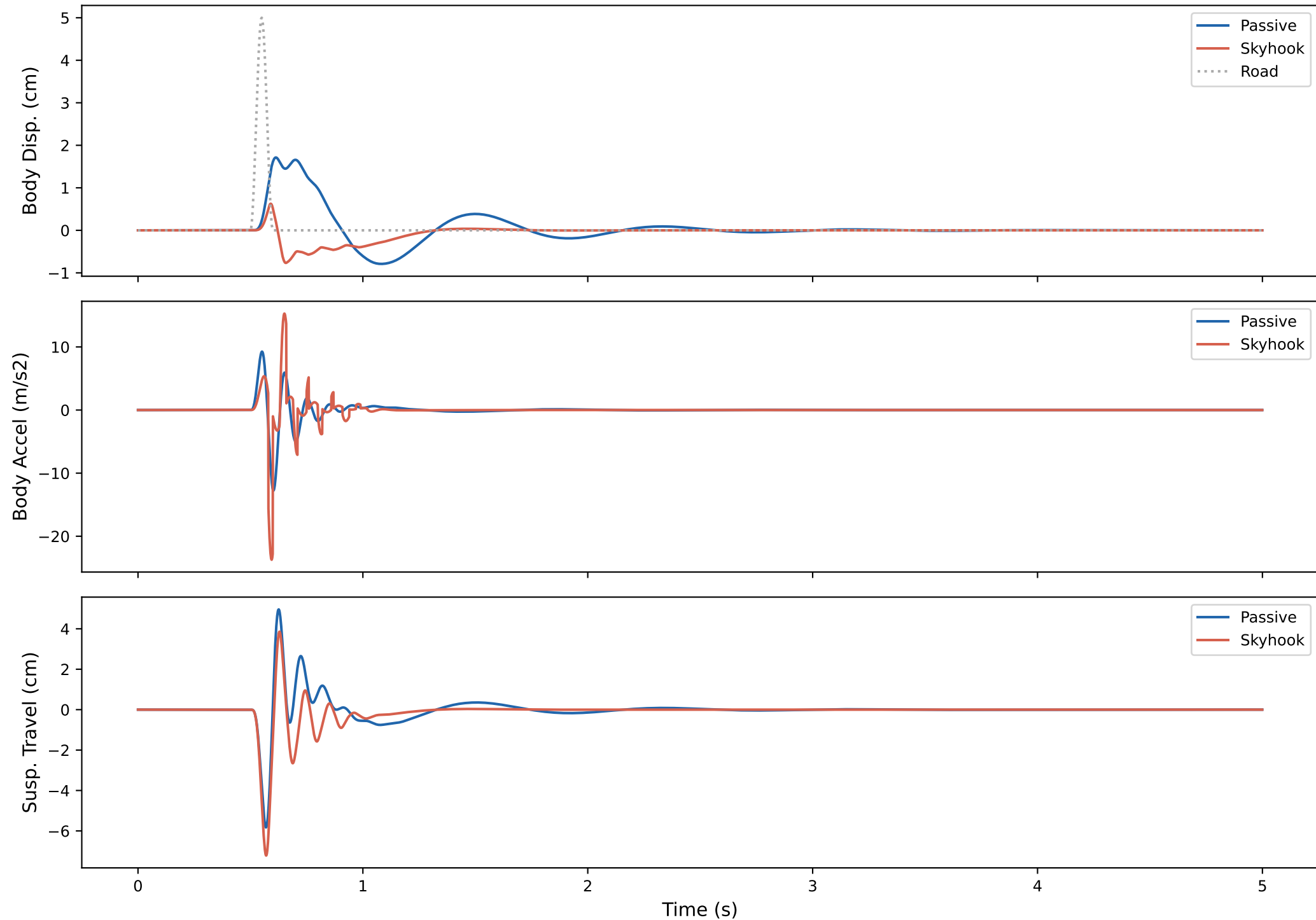
Skyhook vs Passive - Bump (100 Hz ZOH, semi-implicit Euler)
