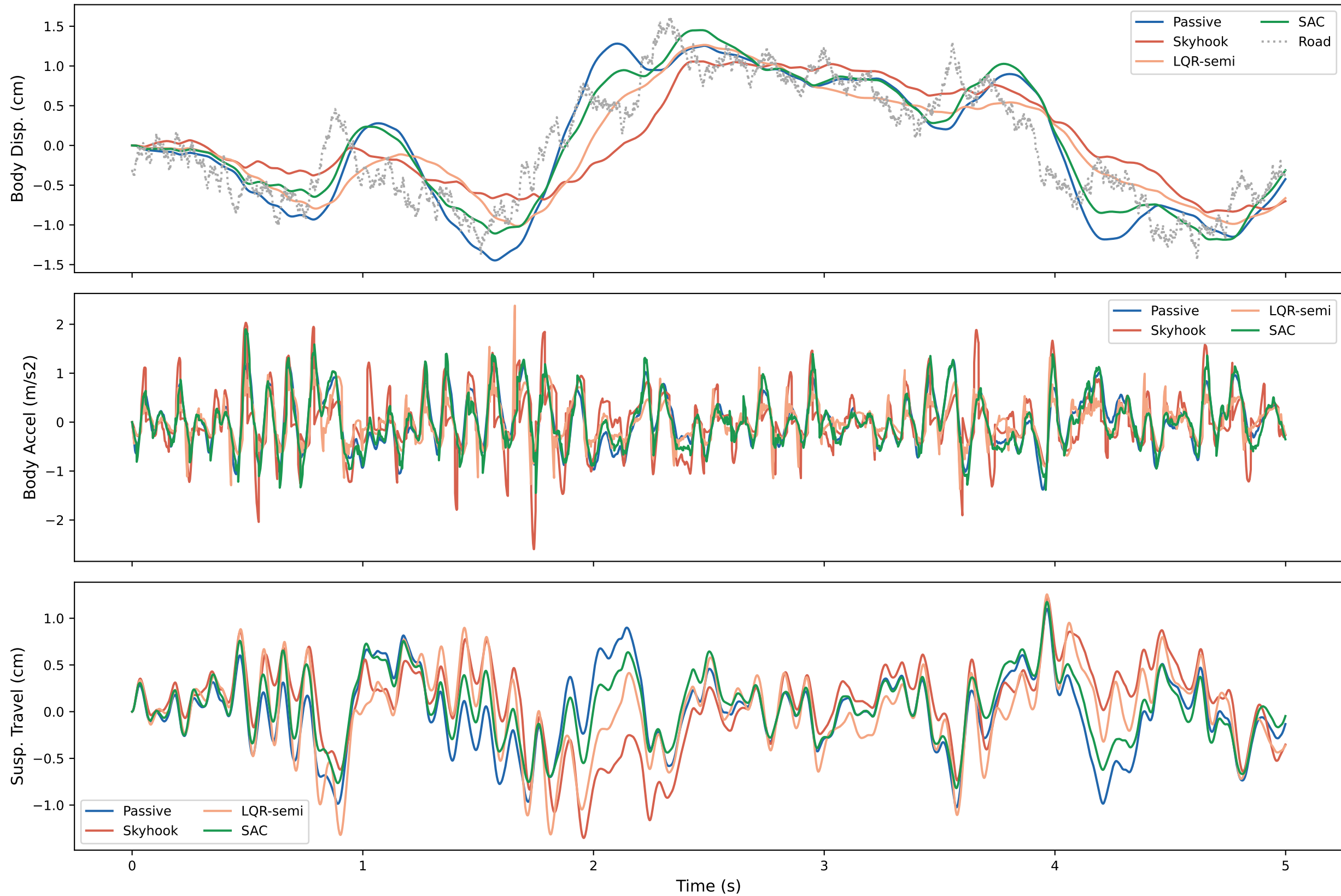
4-Controller Comparison - Random
