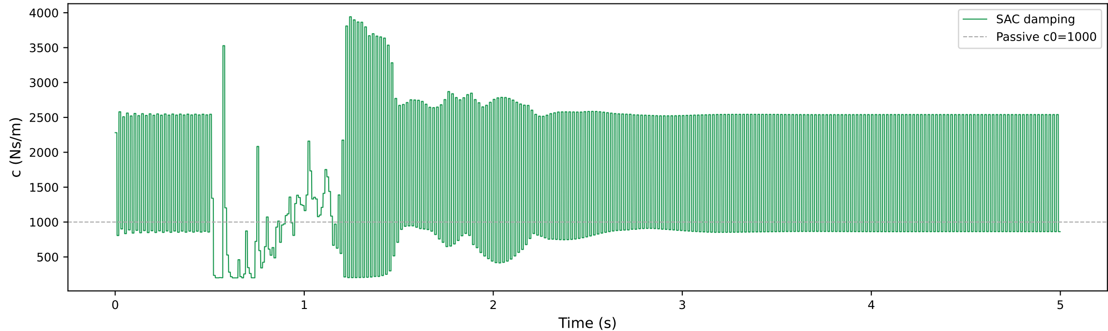
SAC Damping History - Bump
