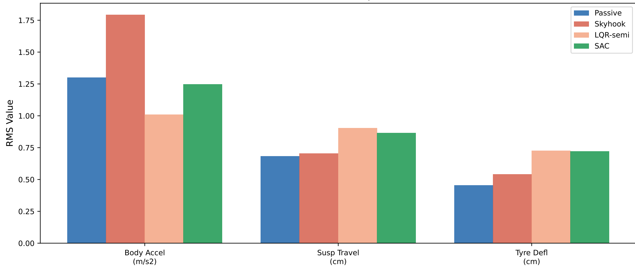
RMS Metrics - Bump Road
