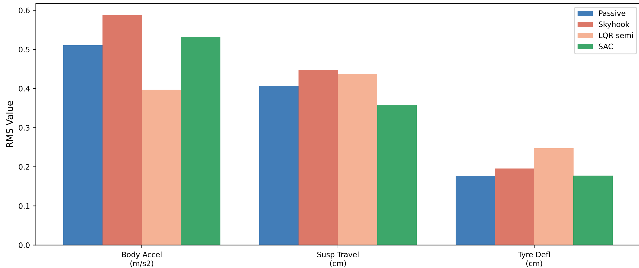
RMS Metrics - Random Road
