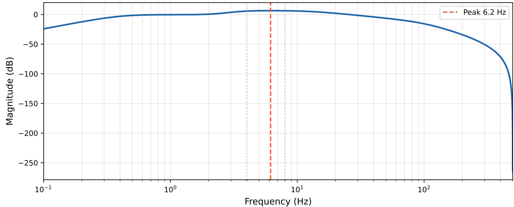
ISO 2631-1 Wk Filter - Magnitude Response
