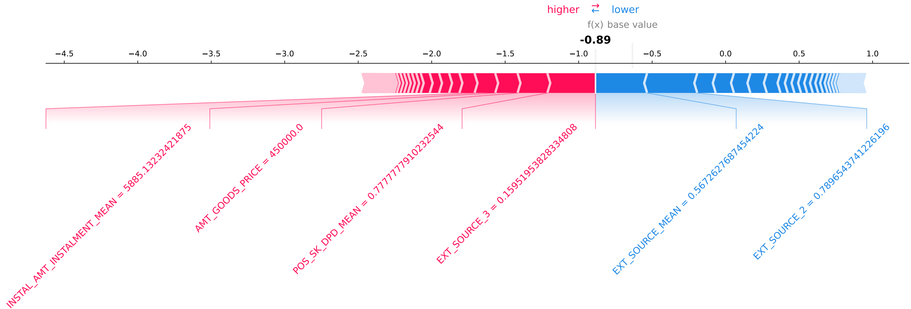
SHAP force plot — SK_ID_CURR 100001 (score=29.2%)
