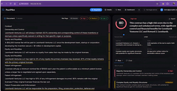
Document Cockpit
