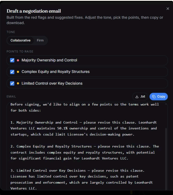
Negotiation Co-pilot
