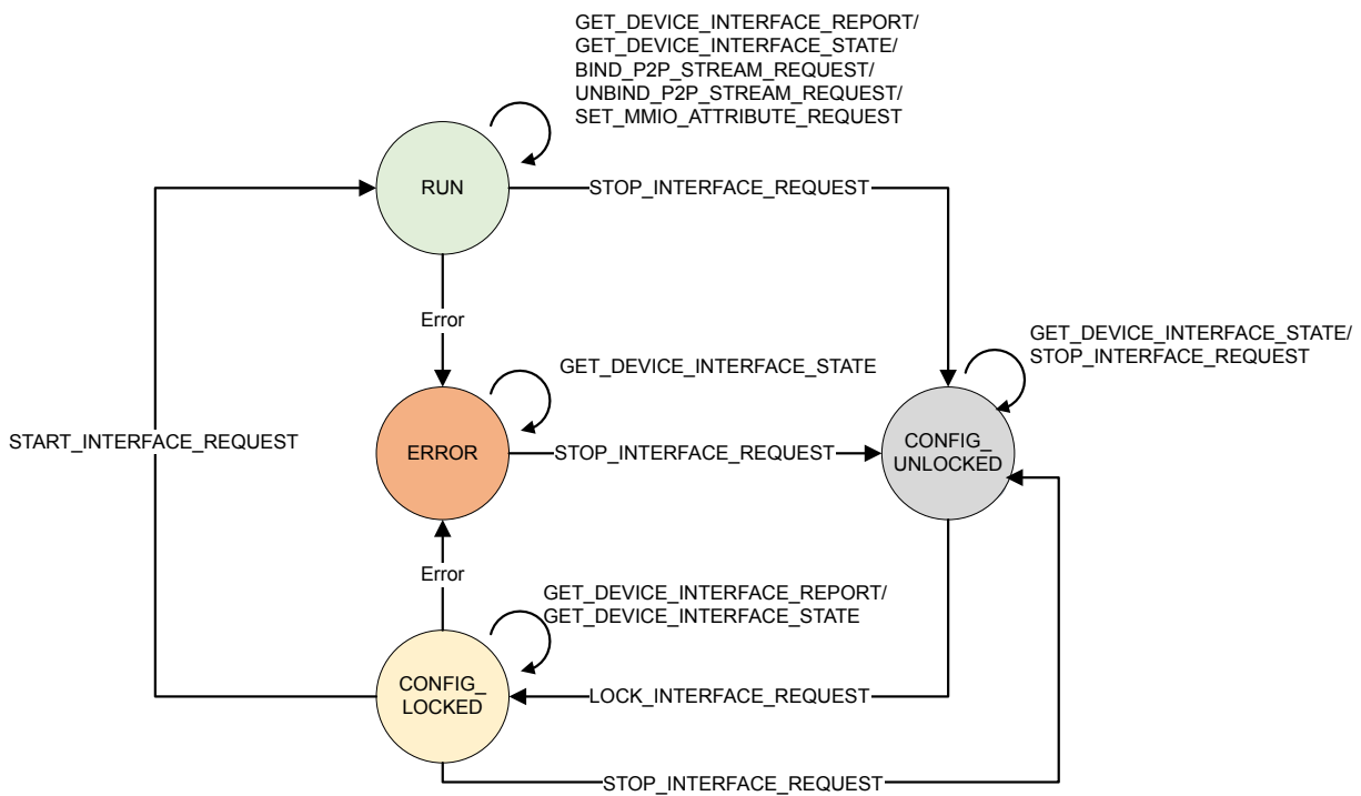
Figure 11-5 TDISP State Machine §
