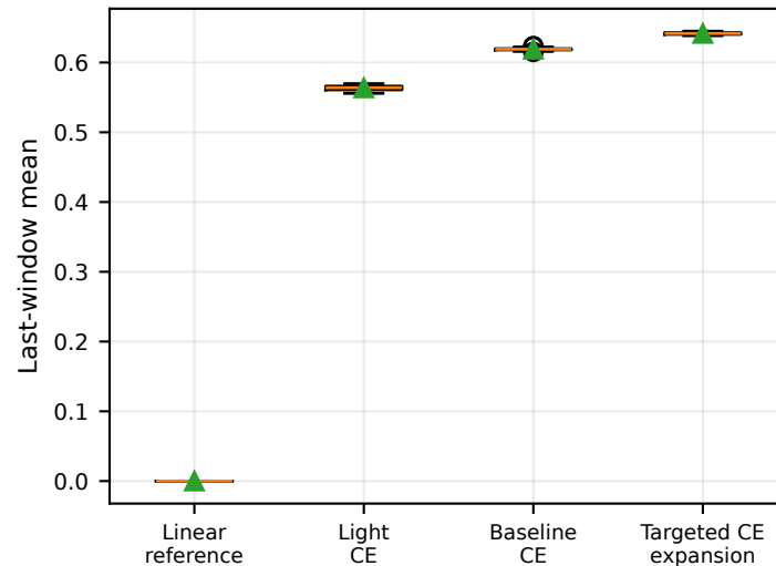
Spatial-advantage Gini (K5)
